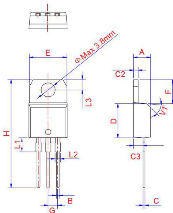
TO-220B Non-Ins
