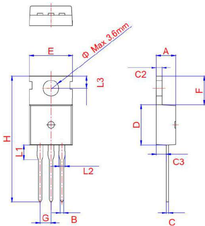
TO-220C
