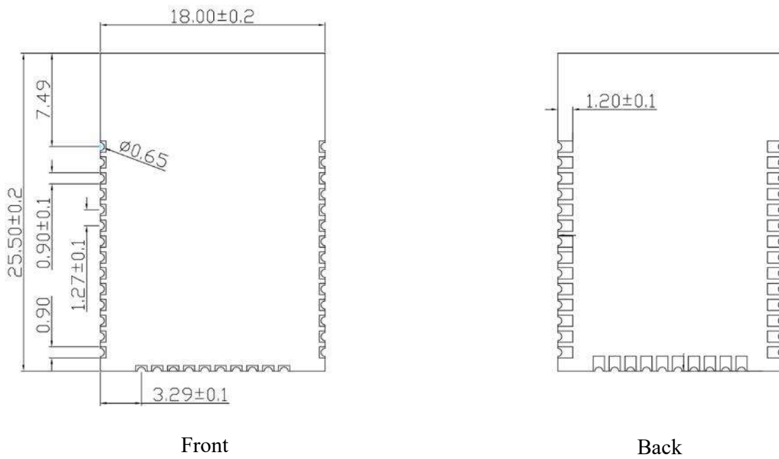
Figure 4 dimension diagram
