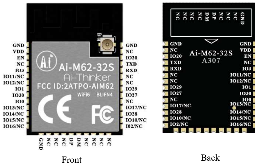
Figure 6 pin diagram
