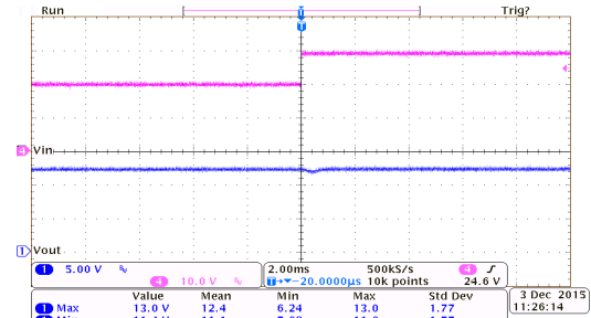
Line Transient Response: HT75C0-7 ( I_{OUT}=10mA )
