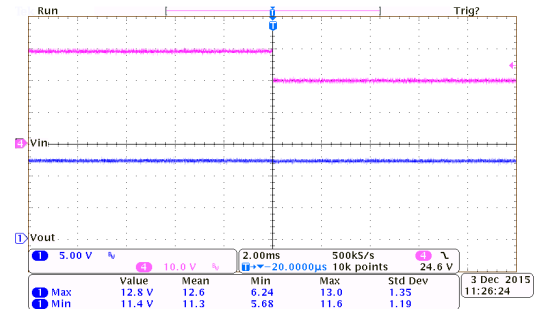
Line Transient Response: HT75C0-7 ( I_{OUT}=10mA )
