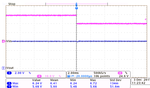
Line Transient Response: HT7560-7 ( I_{OUT}=10mA )
