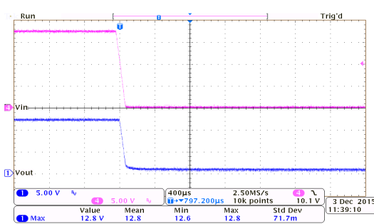
Power Off Response: HT75C0-7 ( I_{OUT}=0mA , T_{FALL}=0.1ms )
