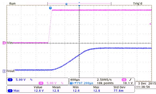
Power On Response: HT75C0-7 ( I_{OUT}=0mA , T_{RISE}=0.1ms )
