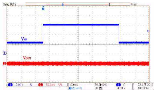
Line Transient Response: HT73L10 ( V_{IN}=2.3V to 6.0V, I_{OUT}=10mA )
