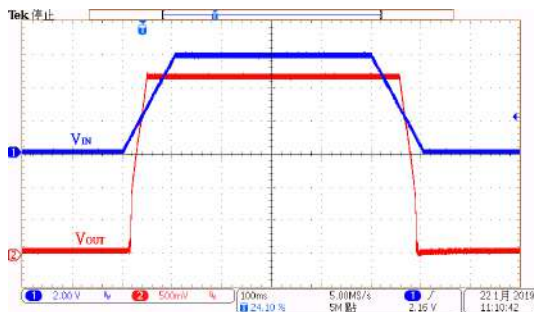
Power On/OFF Response: HT73L27 (V_{IN}=6.0V, I_{OUT}=0mA, T_{RISE}=T_{FALL}=100ms)
