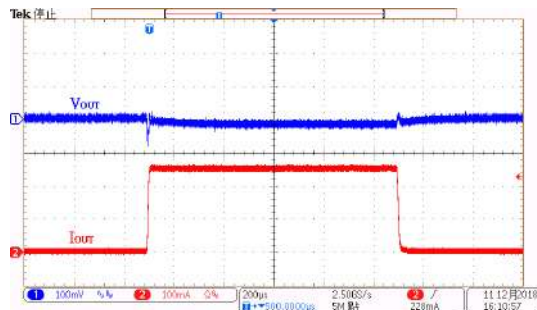
Load Transient Response: HT73L30 ( V_{IN}=4.0V , I_{OUT}=1mA to 250mA )
