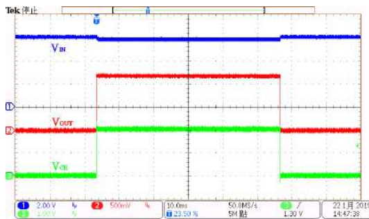
ON/OFF Response: HT73L12 (V_{IN}=6.0V, I_{OUT}=200mA, V_{CE}=0V \text{ to } 2V)
