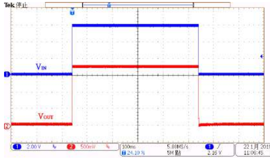
Power On/OFF Response: HT73L18 ( V_{IN}=6.0V , I_{OUT}=0mA , T_{RISE}=T_{FALL}=0.1ms )
