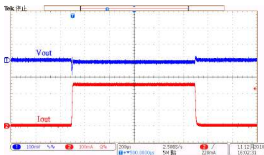
Load Transient Response: HT73L12 (V_{IN}=2.3V, I_{OUT}=1mA \text{ to } 250mA)
