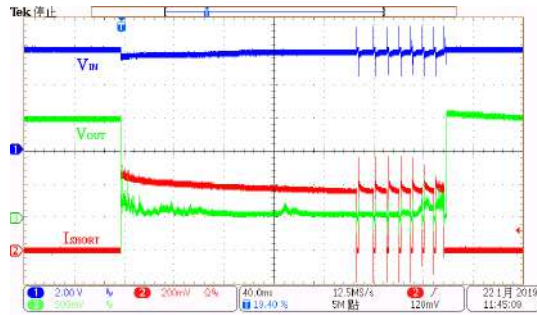
Short Protection: HT73L15 ( V_{IN}=6.0V , V_{OUT} Short)
