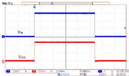
Power On/OFF Response: HT73L12 (V_{IN}=6.0V, I_{OUT}=0mA, T_{RISE}=T_{FALL}=0.1ms)
