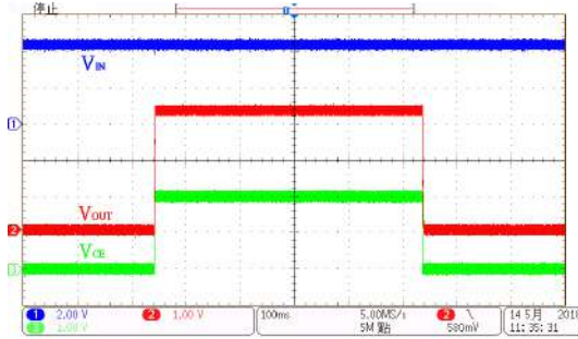
ON/OFF Response: HT73L33 ( V_{IN}=4.3V , I_{OUT}=0mA , V_{CE}=0V to 2V )
