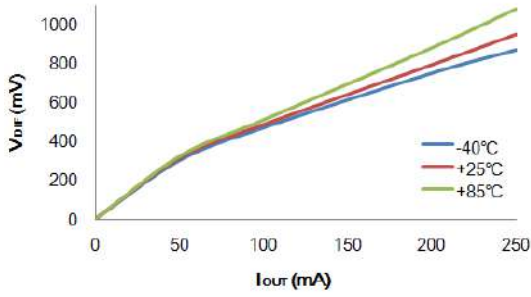
Dropout Voltage: HT73L09
