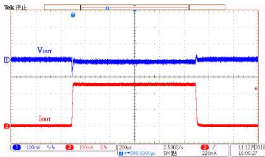
Load Transient Response: HT73L18 ( V_{IN}=2.8V , I_{OUT}=1mA to 250mA )
