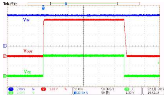
ON/OFF Response: HT73L36 ( V_{IN}=6.0V , I_{OUT}=0mA , V_{CE}=0V to 2V )
