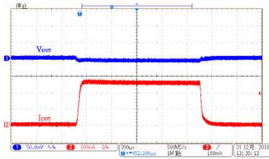
Load Transient Response: HT73L18 ( V_{IN}=6.0V , I_{OUT}=1mA to 250mA )
