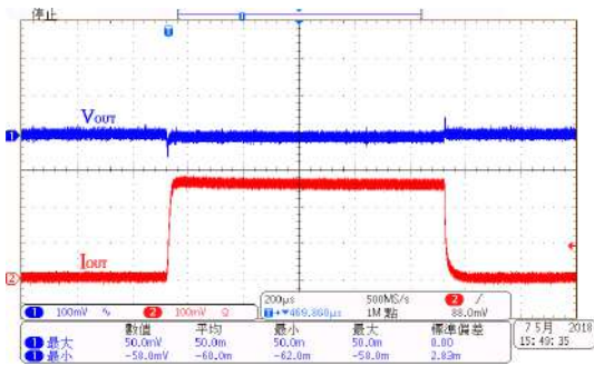
Load Transient Response: HT73L09 ( V_{IN}=2.3V , I_{OUT}=1mA to 250mA)
