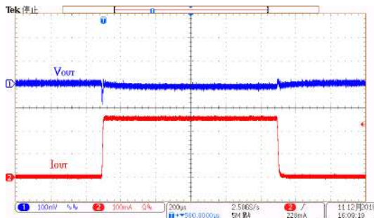
Load Transient Response: HT73L27 ( V_{IN}=3.7V , I_{OUT}=1mA to 250mA )
