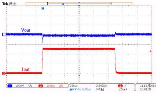
Load Transient Response: HT73L10 ( V_{IN}=2.3V , I_{OUT}=1mA to 250mA)
