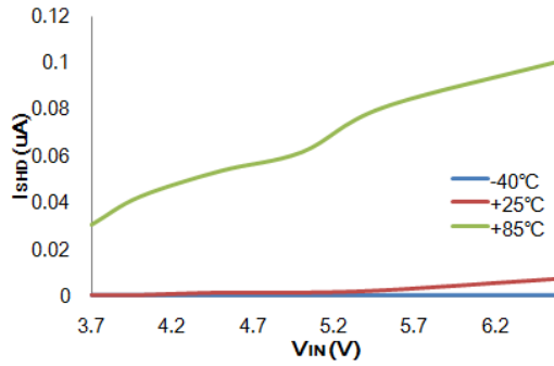
I_{SHD} vs V_{IN} : HT73L27 ( I_{OUT}=0mA )
