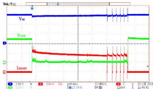
Short Protection: HT73L25 ( V_{IN}=6.0V , V_{OUT} Short)
