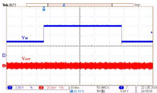
Line Transient Response: HT73L18 ( V_{IN}=2.8V to 6.0V , I_{OUT}=10mA )
