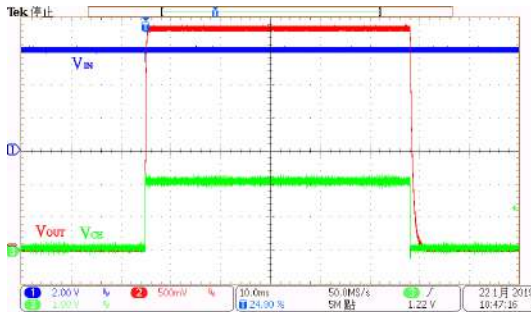
ON/OFF Response: HT73L33 ( V_{IN}=6.0V , I_{OUT}=0mA , V_{CE}=0V to 2V )
