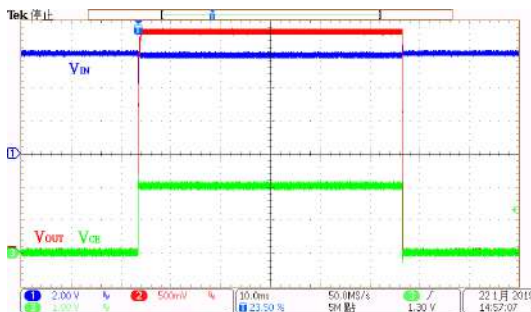
ON/OFF Response: HT73L33 ( V_{IN}=6.0V , I_{OUT}=200mA , V_{CE}=0V to 2V )
