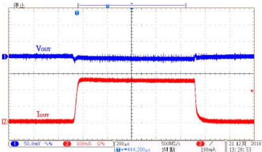
Load Transient Response: HT73L09 ( V_{IN}=6.0V , I_{OUT}=1mA to 250mA)
