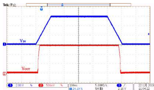
Power On/OFF Response: HT73L15 (V_{IN}=6.0V, I_{OUT}=0mA, T_{RISE}=T_{FALL}=100ms)
