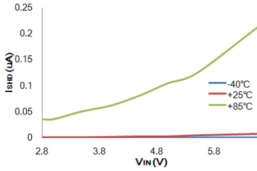
I_{SHD} vs V_{IN} : HT73L18 ( I_{OUT}=0mA )
