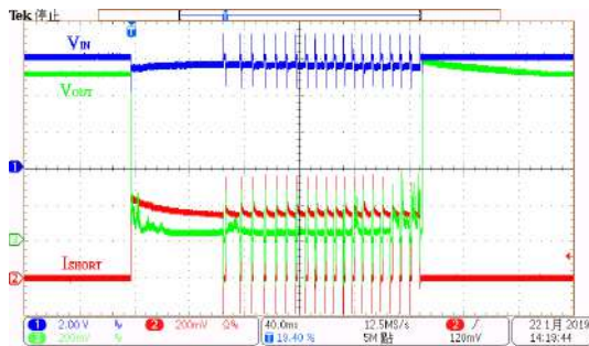
Short Protection: HT73L09 (V_{IN}=6.0V, V_{OUT} \text{ Short})
