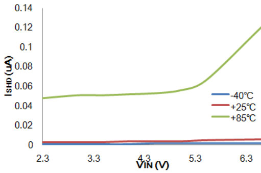
I_{SHD} vs V_{IN} : HT73L09 ( I_{OUT}=0mA )
