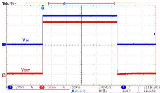
Power On/OFF Response: HT73L27 (V_{IN}=6.0V, I_{OUT}=0mA, T_{RISE}=T_{FALL}=0.1ms)
