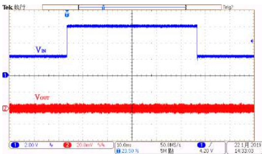
Line Transient Response: HT73L09 ( V_{IN}=2.3V to 6.0V, I_{OUT}=10mA )
