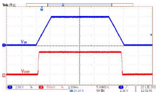
Power On/OFF Response: HT73L12 (V_{IN}=6.0V, I_{OUT}=0mA, T_{RISE}=T_{FALL}=100ms)
