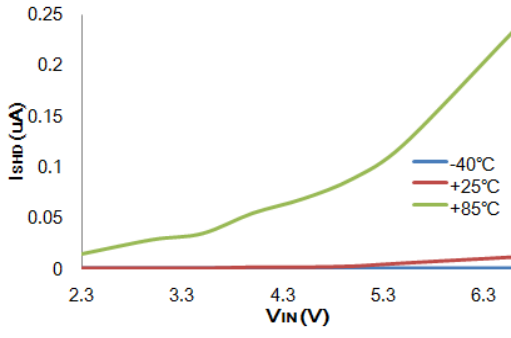
I_{SHD} vs V_{IN} : HT73L12 ( I_{OUT}=0mA )
