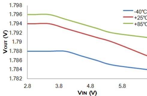
Line Regulation: HT73L18 (I OUT =10mA)
