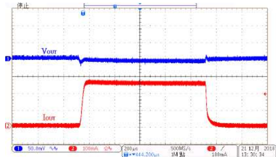
Load Transient Response: HT73L10 ( V_{IN}=6.0V , I_{OUT}=1mA to 250mA)
