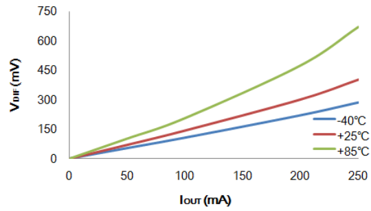
Dropout Voltage: HT73L36
