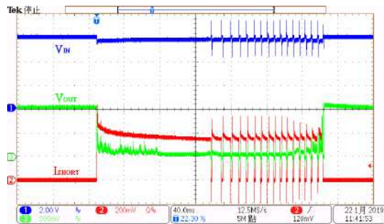
Short Protection: HT73L10 (V_{IN}=6.0V, V_{OUT} \text{ Short})
