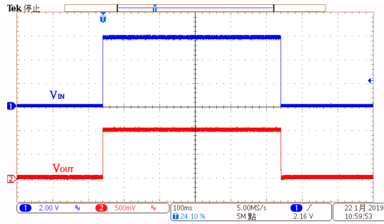
Power On/OFF Response: HT73L10 (V_{IN}=6.0V, I_{OUT}=0mA, T_{RISE}=T_{FALL}=0.1ms)
