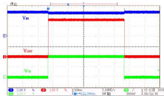
ON/OFF Response: HT73L36 ( V_{IN}=4.6V , I_{OUT}=200mA , V_{CE}=0V to 2V )
