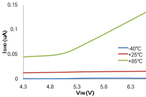
I_{SHD} vs V_{IN} : HT73L33 ( I_{OUT}=0mA )
