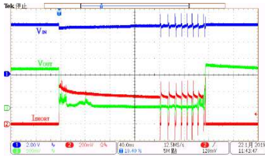
Short Protection: HT73L12 ( V_{IN}=6.0V , V_{OUT} Short)
