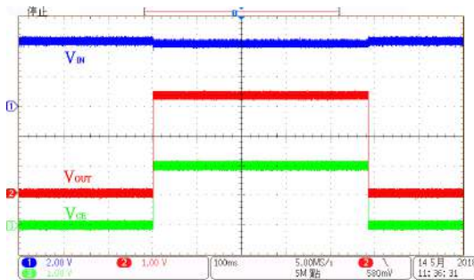
ON/OFF Response: HT73L33 ( V_{IN}=4.3V , I_{OUT}=200mA , V_{CE}=0V to 2V )
