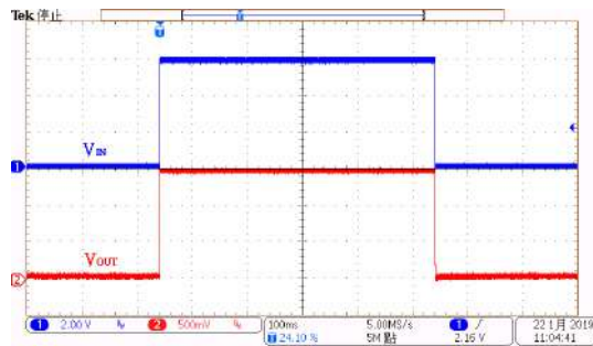
Power On/OFF Response: HT73L15 (V_{IN}=6.0V, I_{OUT}=0mA, T_{RISE}=T_{FALL}=0.1ms)
