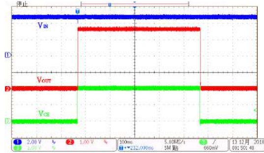
ON/OFF Response: HT73L36 ( V_{IN}=4.6V , I_{OUT}=0mA , V_{CE}=0V to 2V )
