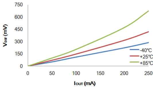
Dropout Voltage: HT73L33
