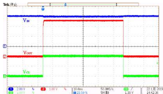
ON/OFF Response: HT73L36 ( V_{IN}=6.0V , I_{OUT}=200mA , V_{CE}=0V to 2V )
