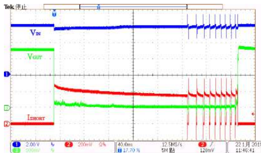
Short Protection: HT73L18 ( V_{IN}=6.0V , V_{OUT} Short)
