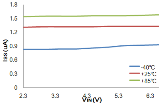
I_{SS} vs V_{IN} : HT73L09 ( I_{OUT}=0mA )
