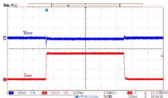
Load Transient Response: HT73L15 (V_{IN}=2.5V, I_{OUT}=1mA \text{ to } 250mA)
