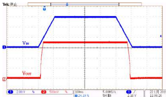
Power On/OFF Response: HT73L18 ( V_{IN}=6.0V , I_{OUT}=0mA , T_{RISE}=T_{FALL}=100ms )
