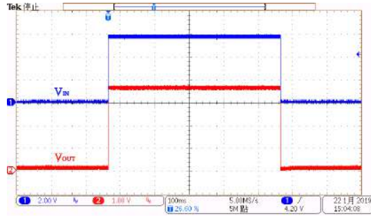
Power On/OFF Response: HT73L36 ( V_{IN}=6.0V , I_{OUT}=0mA , T_{RISE}=T_{FALL}=0.1ms )
