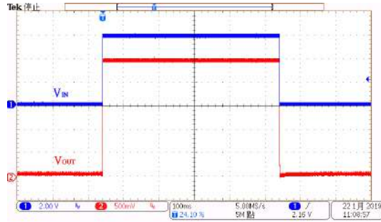
Power On/OFF Response: HT73L25 ( V_{IN}=6.0V , I_{OUT}=0mA , T_{RISE}=T_{FALL}=0.1ms )
