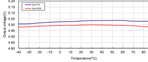
Output Voltage vs Temperature: HT7150-2
