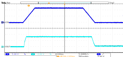
Power ON/OFF Response: HT7133-2 (V IN =12V, I OUT =0mA, TRISE=TFALL=100ms)
