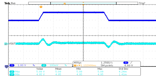
Line Transient Response: HT7150-2 (V IN =6V~7V, I OUT =10mA)
