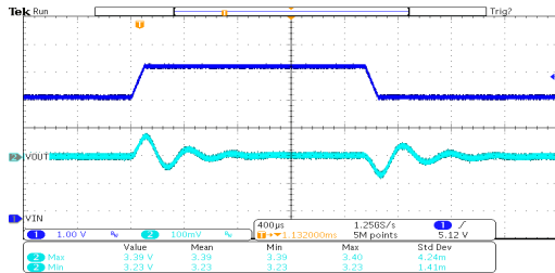
Line Transient Response: HT7133-2 (V IN =4.3V~5.3V, I OUT =10mA)
