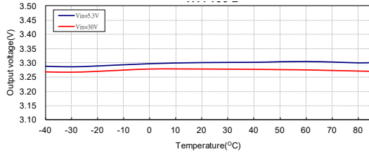
Output Voltage vs Temperature: HT7133-2
