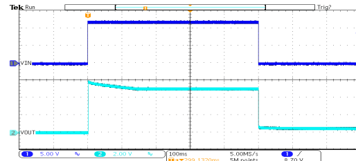
Power ON/OFF Response: HT7150-2 (V IN =12V, I OUT =0mA, TRISE=TFALL=0.1ms)
