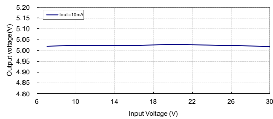
Output Voltage vs Input Voltage: HT7150-2
