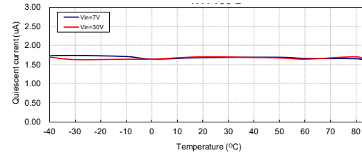
Quiescent Current vs Temperature: HT7150-2 (I OUT =0mA)
