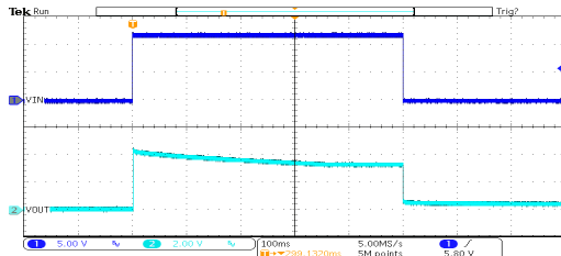
Power ON/OFF Response: HT7133-2 (V IN =12V, I OUT =0mA, TRISE=TFALL=0.1ms)
