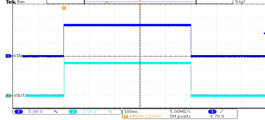
Power ON/OFF Response: HT7150-2 ( V_{IN}=12V , I_{OUT}=30mA , TRISE=TFALL=0.1ms )
