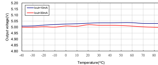
Output Voltage vs Temperature: HT7150-2 (V IN =V OUT +2V)
