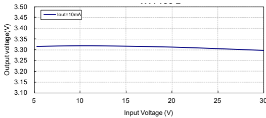
Output Voltage vs Input Voltage: HT7133-2
