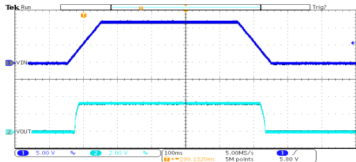
Power ON/OFF Response: HT7133-2 ( V_{IN}=12V , I_{OUT}=30mA , TRISE=TFALL=100ms )
