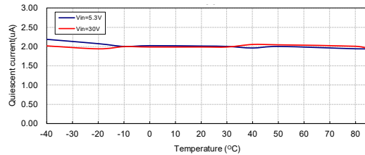
Quiescent Current vs Temperature: HT7133-2 (I OUT =0mA)
