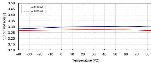
Output Voltage vs Temperature: HT7133-2 (V IN =V OUT +2V)
