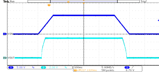
Power ON/OFF Response: HT7150-2 ( V_{IN}=12V , I_{OUT}=30mA , TRISE=TFALL=100ms )
