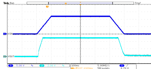
Power ON/OFF Response: HT7150-2 (V IN =12V, I OUT =0mA, TRISE=TFALL=100ms)
