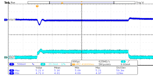
Load Transient Response: HT7150-2 (V IN =7V, I OUT =0mA~15mA)
