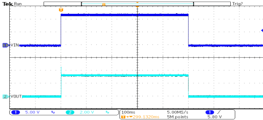
Power ON/OFF Response: HT7133-2 ( V_{IN}=12V , I_{OUT}=30mA , TRISE=TFALL=0.1ms )
