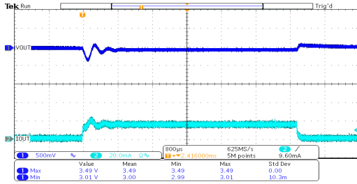
Load Transient Response: HT7133-2 (V IN =5.3V, I OUT =0mA~15mA)
