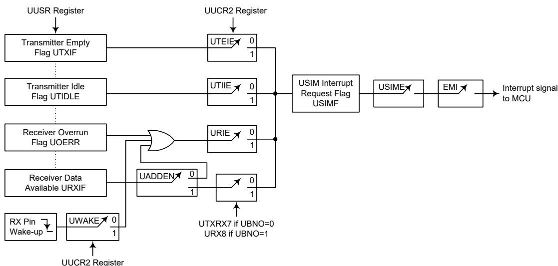
UART Interface Interrupt Structure
