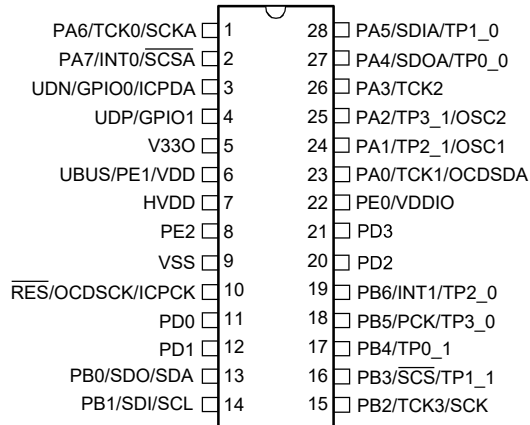
HT68FB560/HT68VB560 28 SSOP-A
