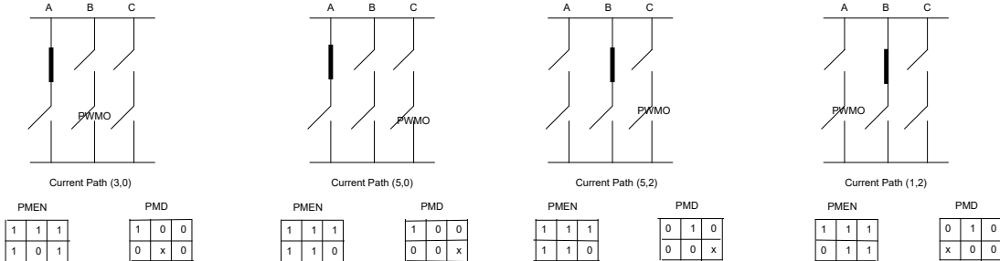
Mask Independent Mode Example
