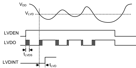
LVD Operation
