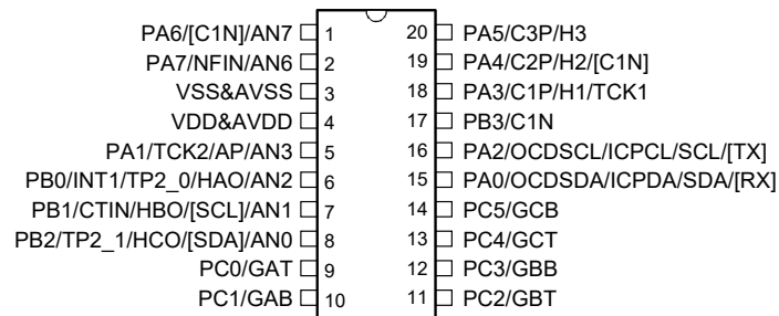
HT66FM5240 20 SSOP-A
