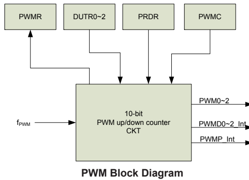
PWM Block Diagram
