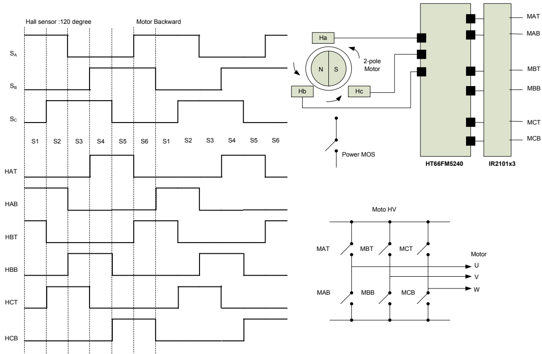
Motor Drive Signal Timing Diagram – Backward Direction
