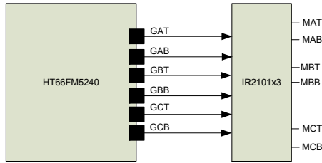
Drive Signal Block Diagram
