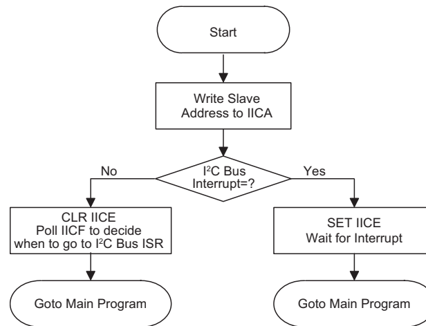
I 2 C Bus Initialisation Flow Chart
