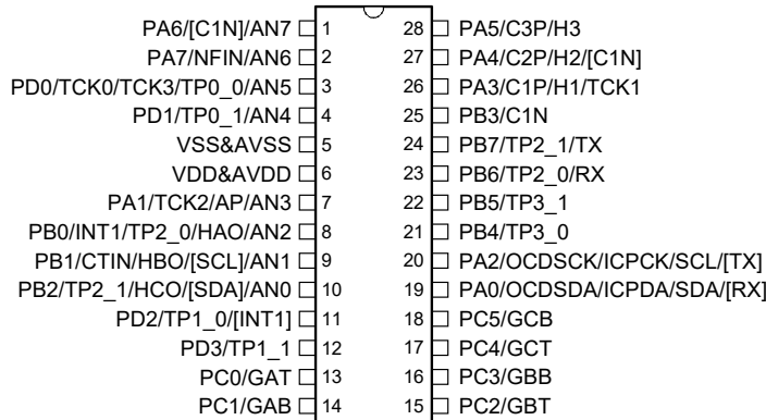
HT66FM5240 28 SSOP-A
