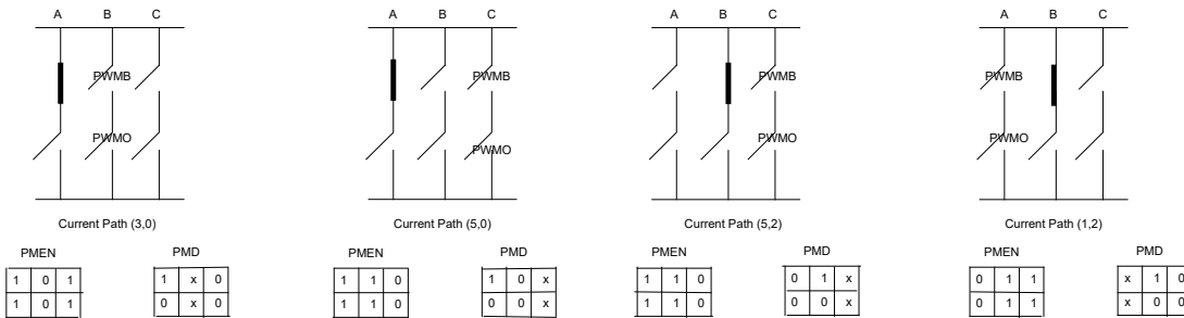
Mask Independent Mode Example
