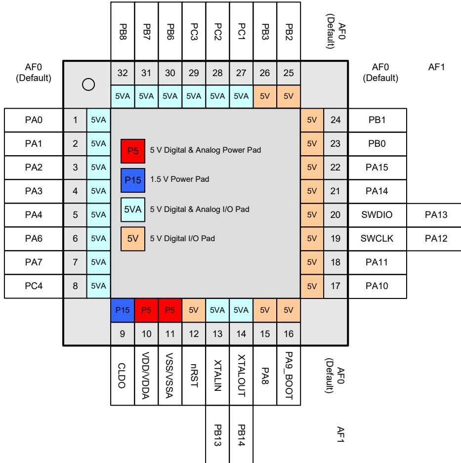
Figure 5. 32-pin QFN Pin Assignment
