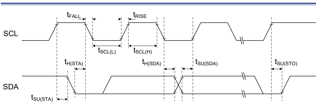
Figure 8. I 2 C Timing Diagram
