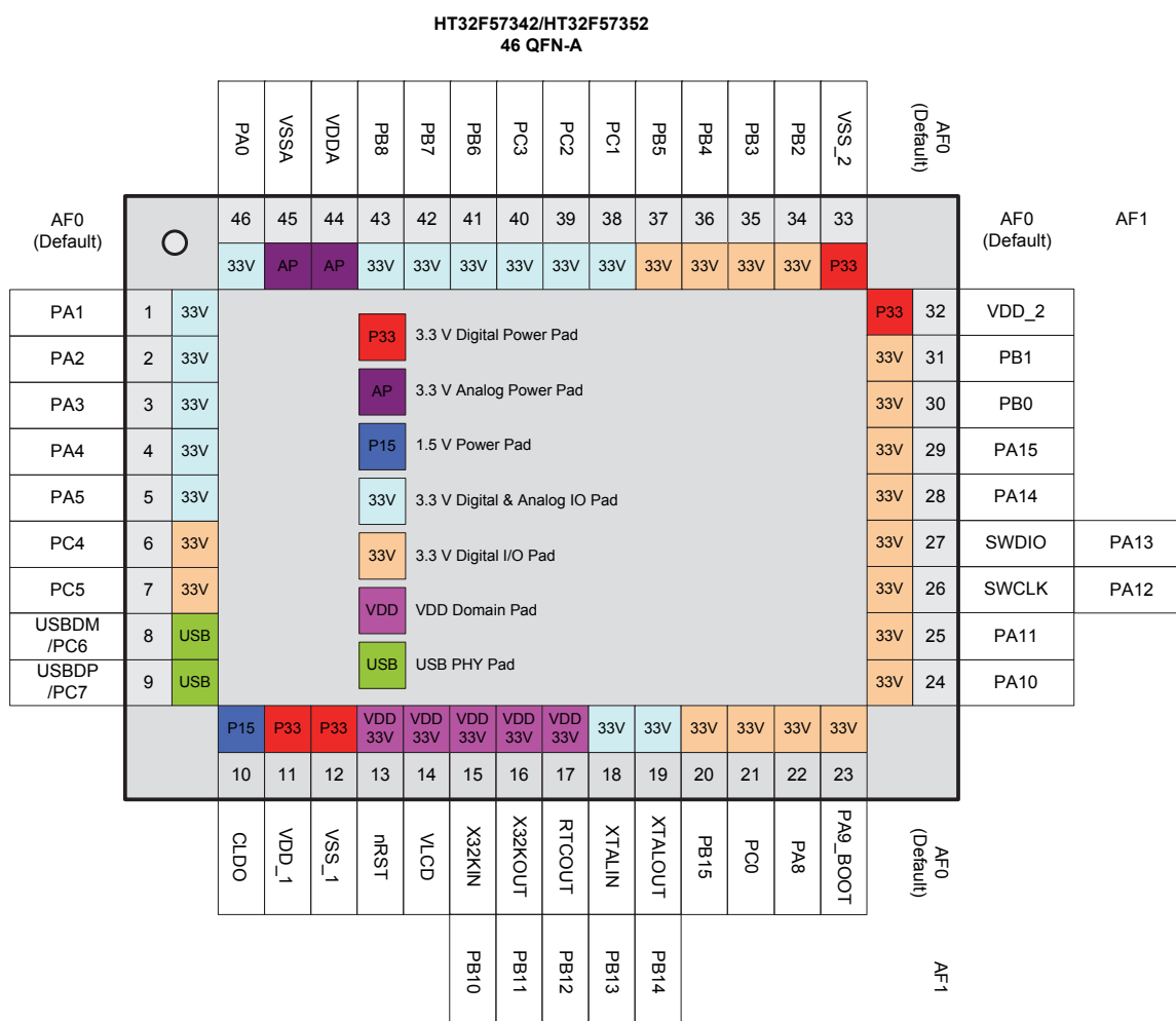
Figure 7. HT32F57342/HT32F57352 46-pin QFN Pin Assignment
