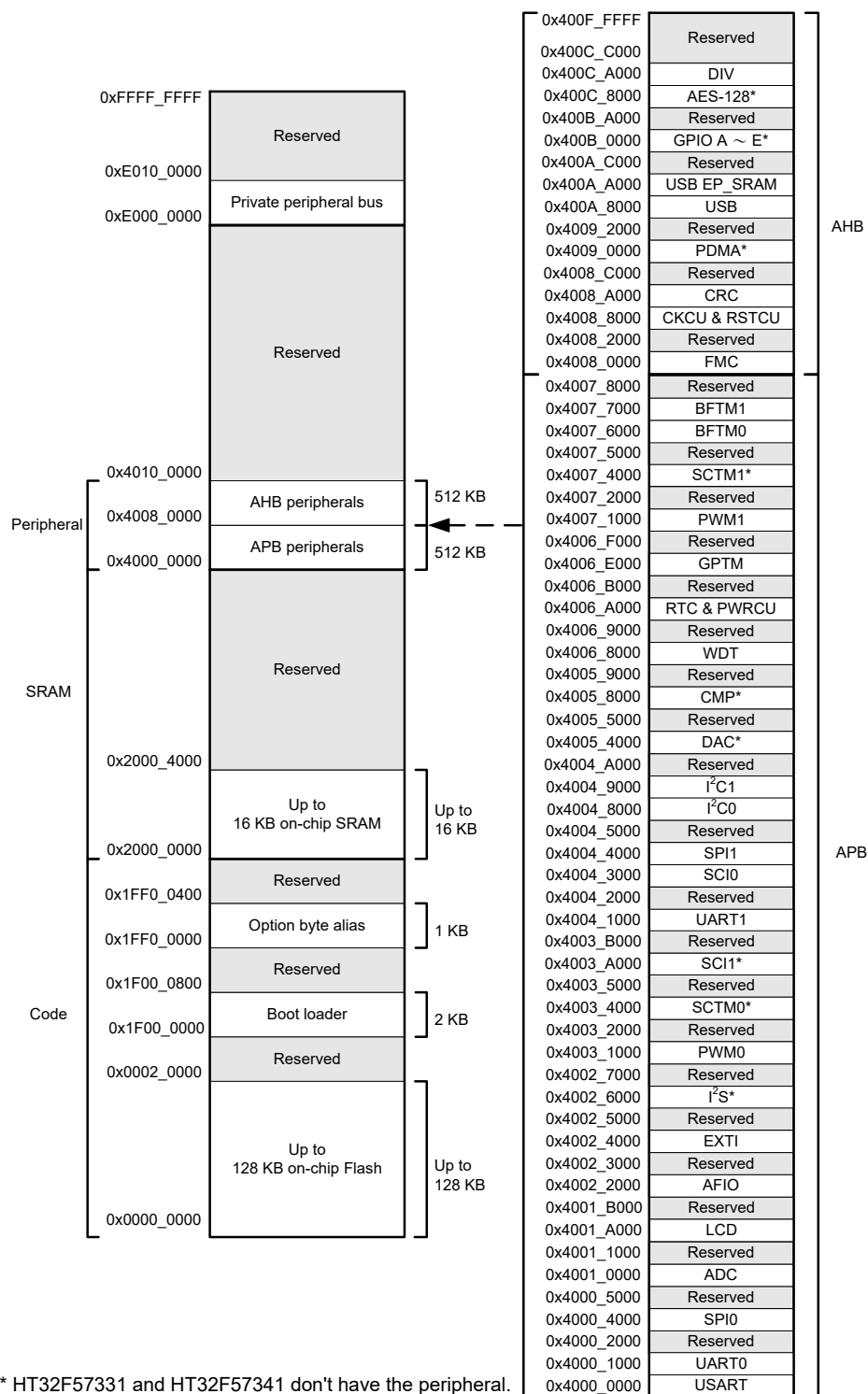
Figure 2. Memory Map
