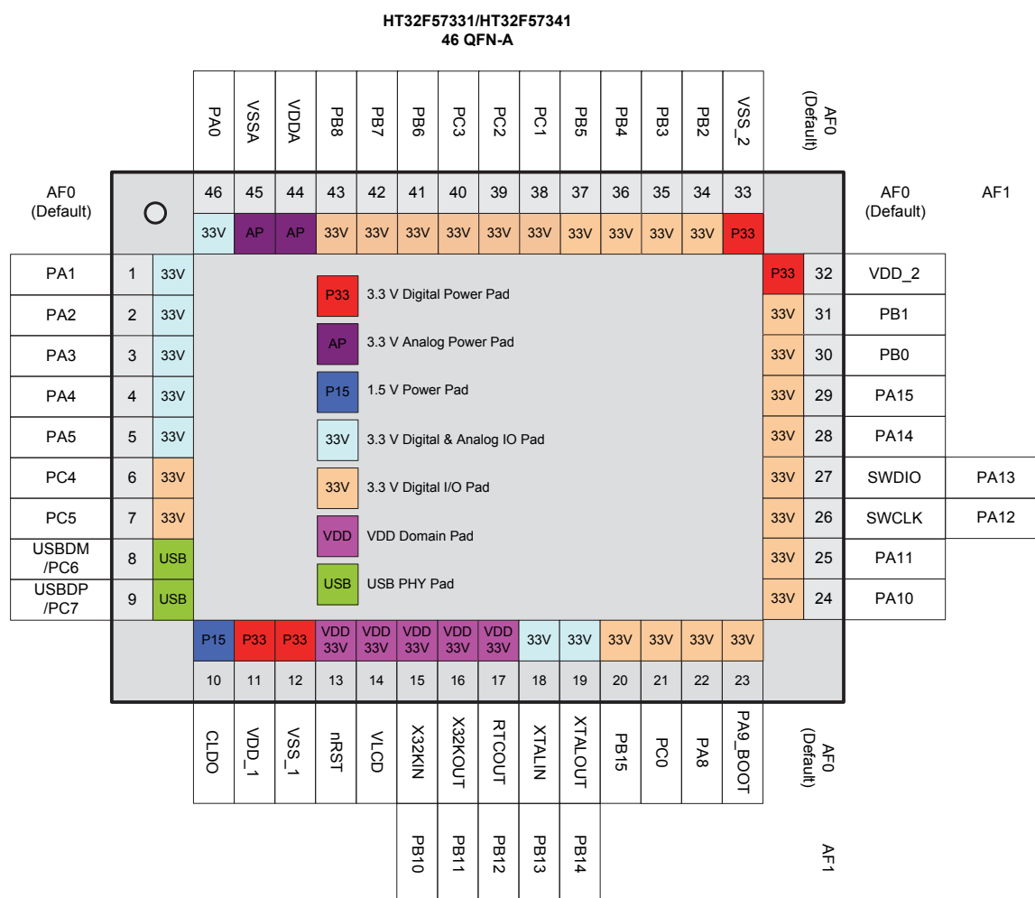
Figure 4. HT32F57331/HT32F57341 46-pin QFN Pin Assignment
