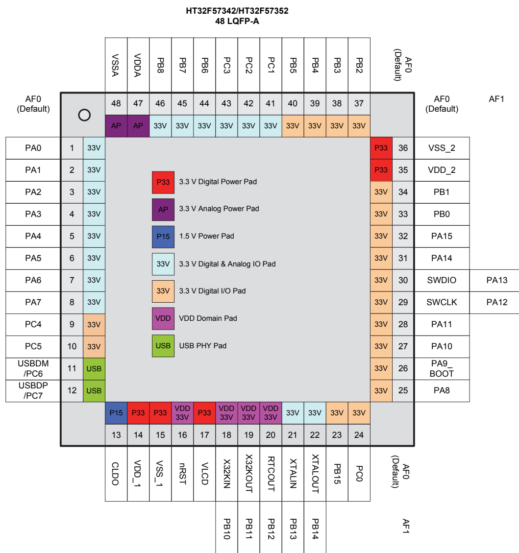
Figure 8. HT32F57342/HT32F57352 48-pin LQFP Pin Assignment
