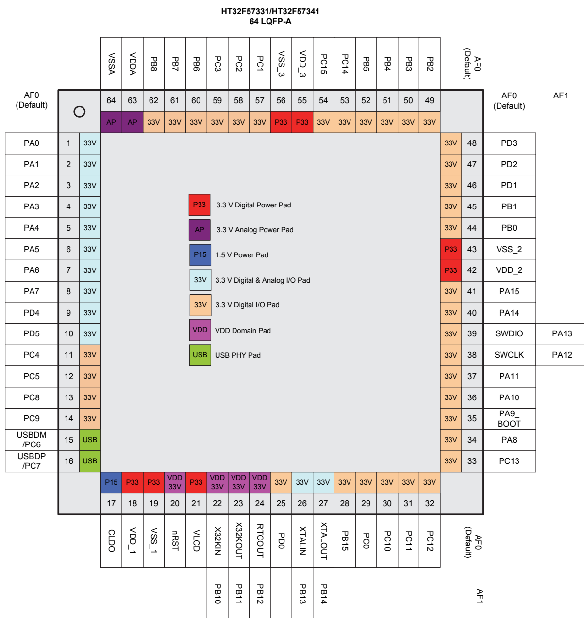
Figure 6. HT32F57331/HT32F57341 64-pin LQFP Pin Assignment
