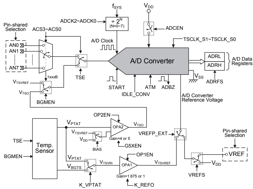
A/D Converter with Temperature Sensor Diagram
