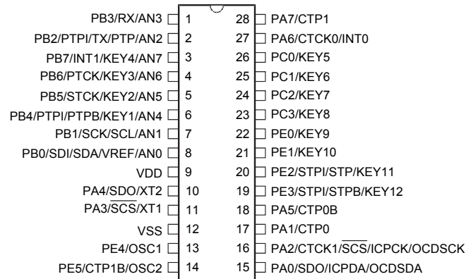
BS66F340/BS66V340 28 SSOP-A
