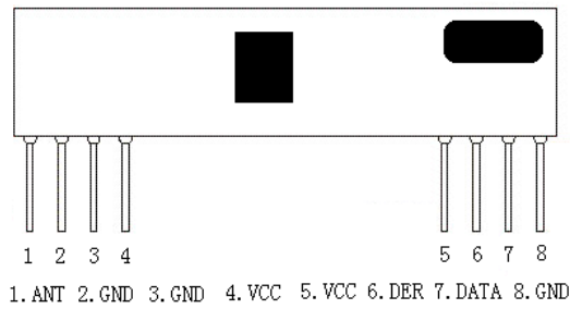
Figure1 RXB6-V1.1Shape & Pins
