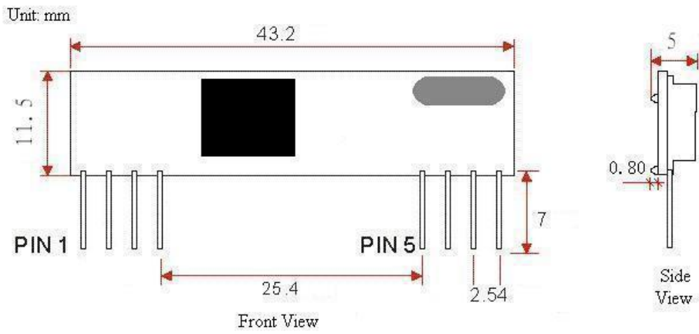
Figure2 RXB6-V1.1 Dimension
