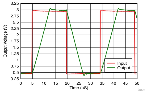
Figure 6-32. Voltage Follower Large Signal Response (50 pF)
