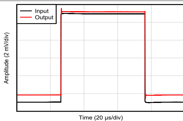
Figure 6-22. Overload Recovery (Positive Rail)
