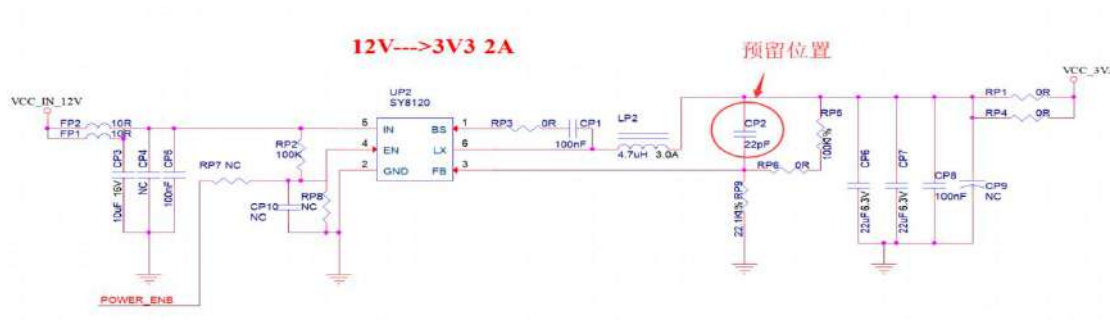
Figure 10 DC-DC step-down circuit diagram
