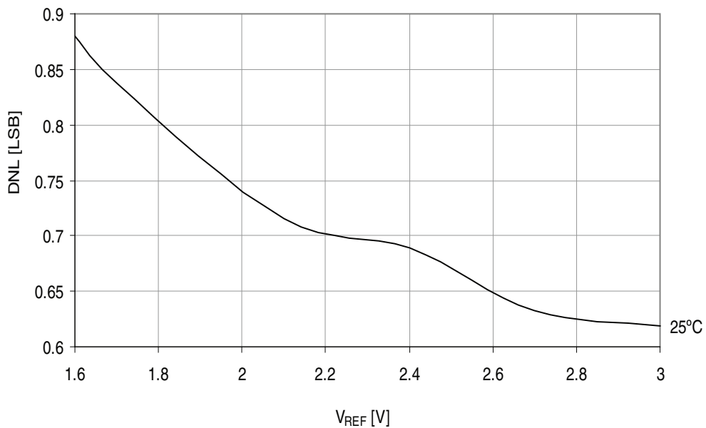
Figure 37-302. DNL error vs. V_{REF}
