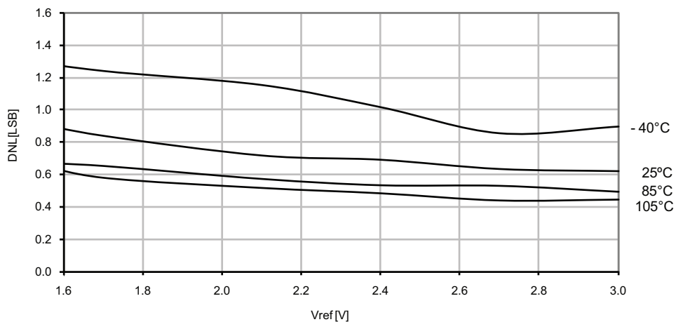
Figure 37-50. DNL error vs. V_{REF} .
