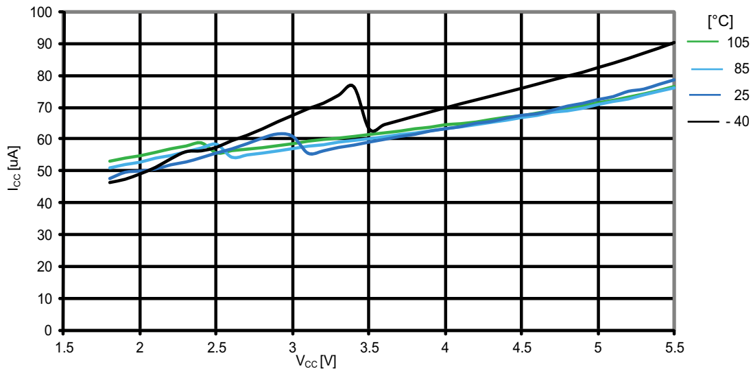
Figure 31-36. ATmega164PA: Analog comparator current vs. V_{CC}
