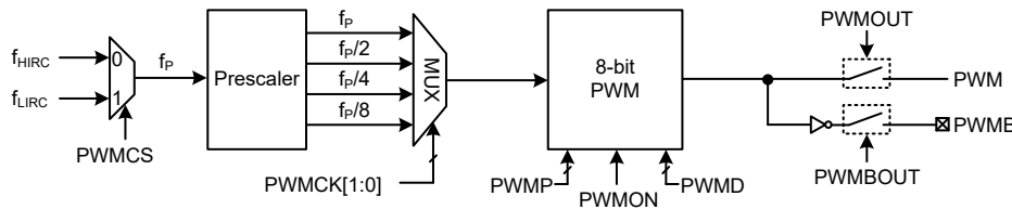
PWM Block Diagram
