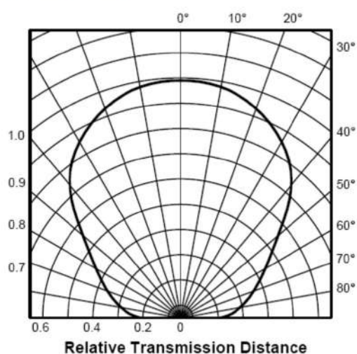
[ Fig.7 ] Directivity
