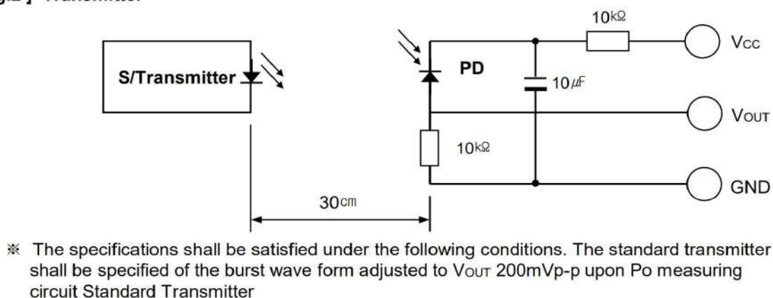
[ Fig.2 ] Transmitter
