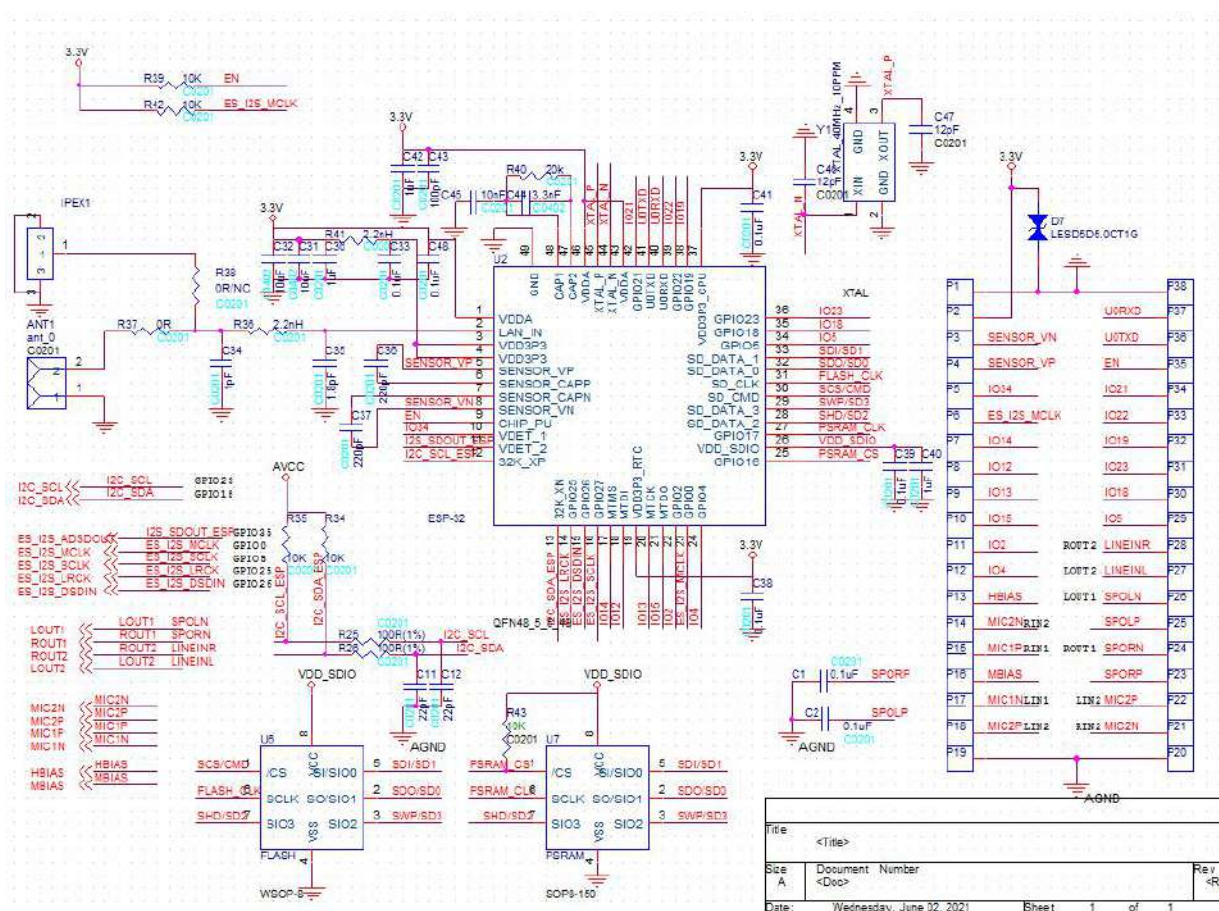
Figure 6 Audio part schematic
