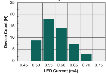
Typical I F for Switch Dropout (N=50, I L =120mA)
