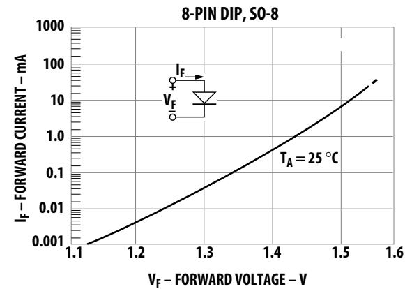
Figure 5: Typical Input Diode Forward Characteristic
