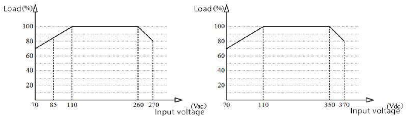
Input voltage and load characteristics curve
