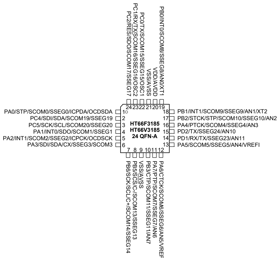
HT66F3185/HT66V3185 24 SOP-A/SSOP-A
