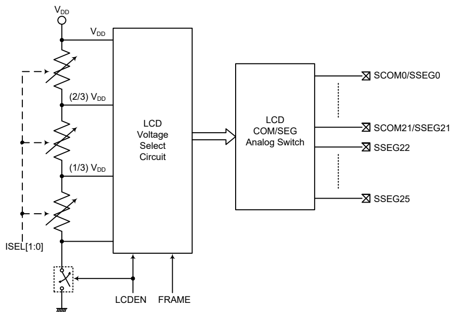
Software Controlled LCD Driver Structure
