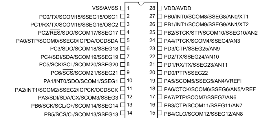
HT66F3185/HT66V3185 28 SOP-A/SSOP-A
