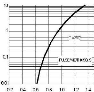
FIG.3 – TYPICAL FORWARD VOLTAGE CHARACTERISTICS PER LEG
