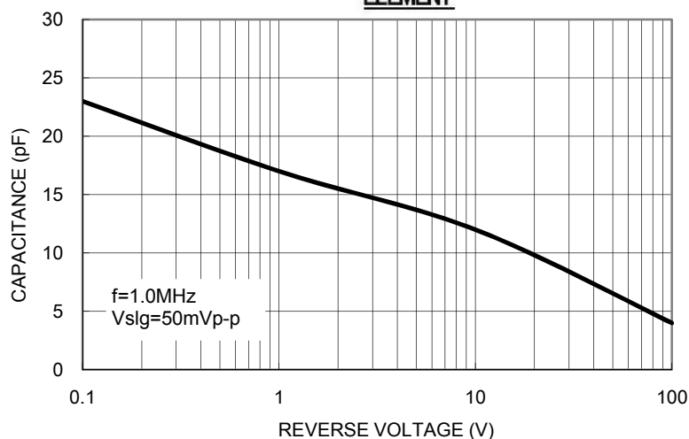
FIG.5 – TYPICAL JUNCTION CAPACITANCE PER ELEMENT
