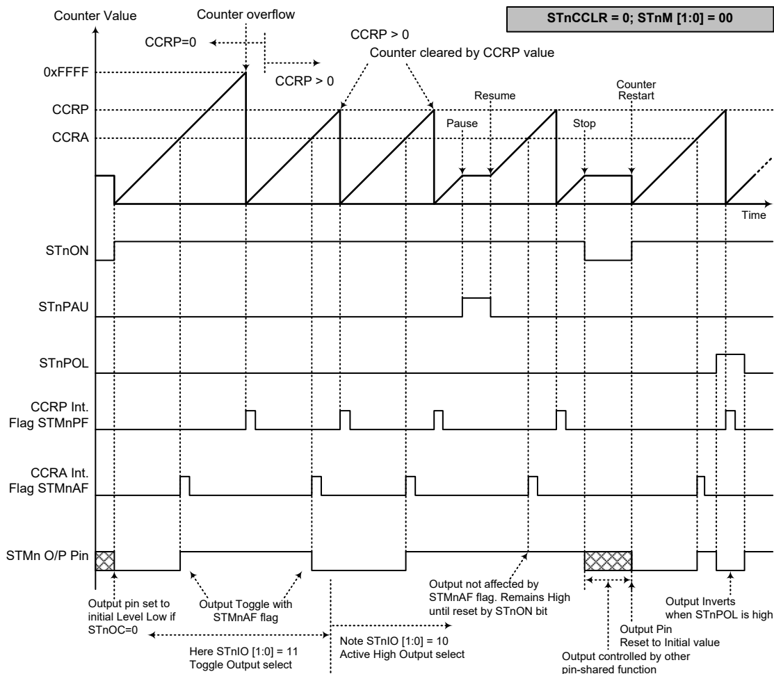
Compare Match Output Mode – STnCCLR=0
