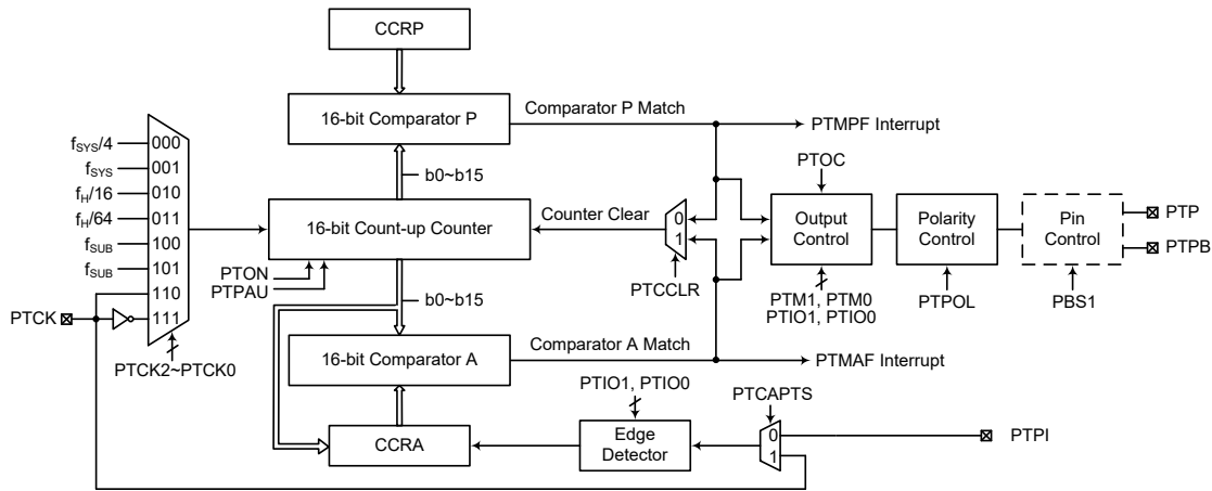
16-bit Periodic Type TM Block Diagram
