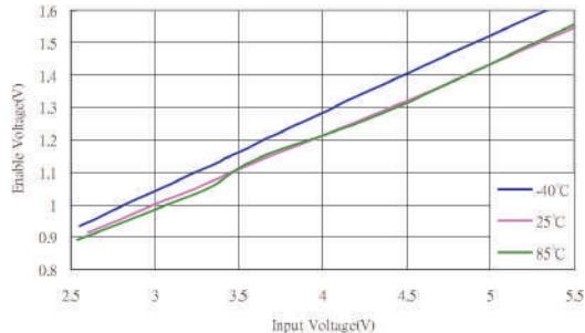
Fig.7 Enable Voltage VS Input Voltage
