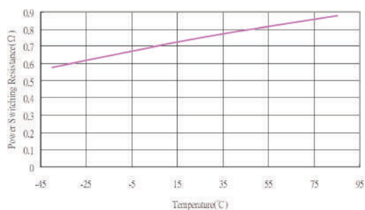
Fig.8 R DS(ON) VS Temperature
