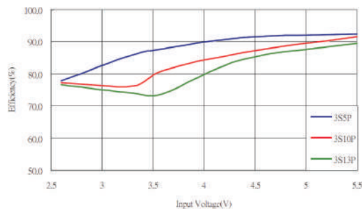
Fig.1 Efficiency VS Input Voltage
