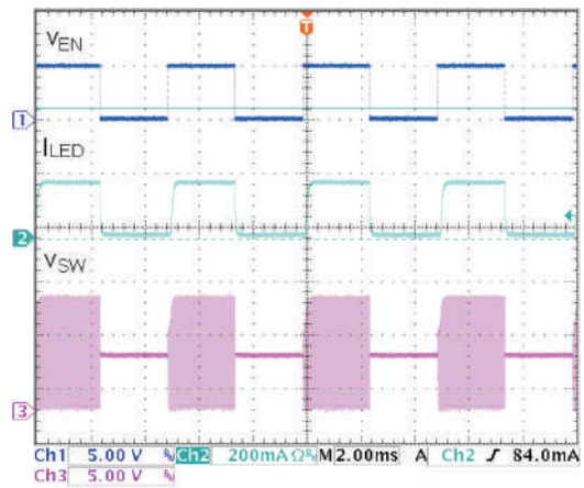
Fig.11 200Hz PWM Dimming Waveform
