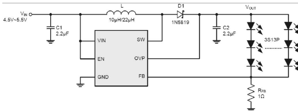
Fig.12 Application Circuits for Driving 39 WLEDs
