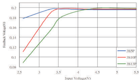
Fig.5 Feedback Voltage VS Input Voltage
