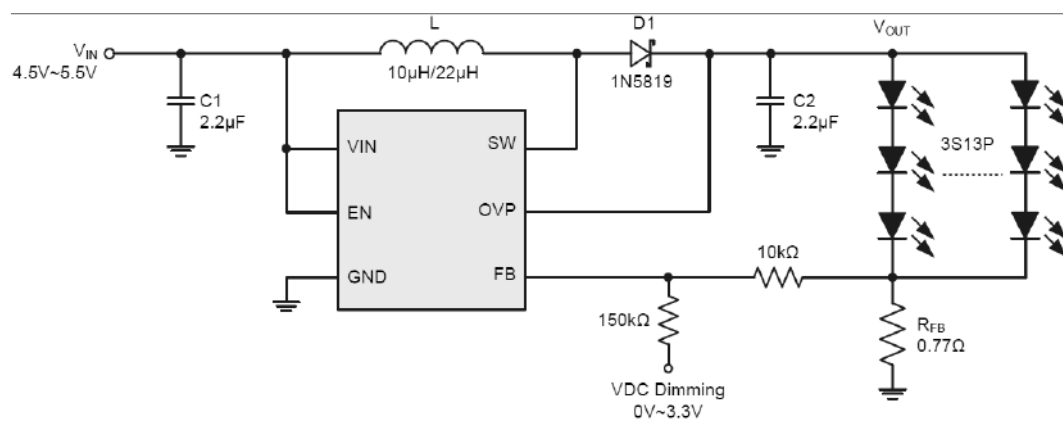
Fig.14 Application Circuit for Dimming Control Using a DC Voltage
