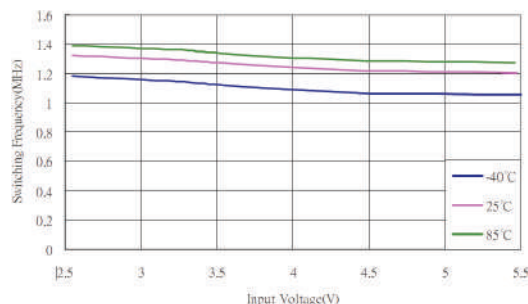
Fig.2 Switching Frequency VS Input Voltage
