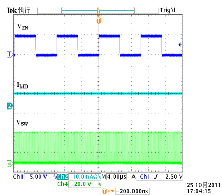
Fig.12 1kHz PWM Dimming Waveform
