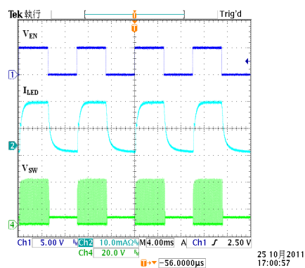
Fig.11 200Hz PWM Dimming Waveform
