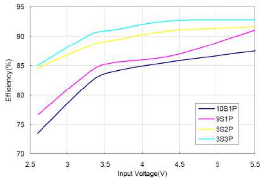
Fig.1 Efficiency VS Input Voltage (L=10μH)
