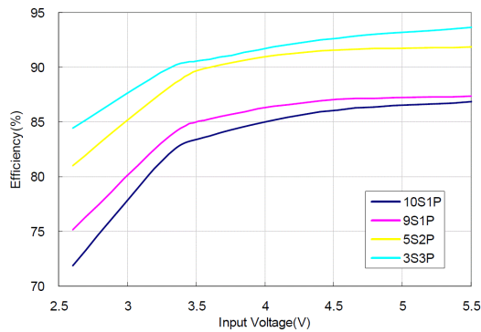
Fig.2 Efficiency VS Input Voltage (L=22μH)
