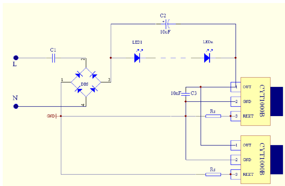
Parallel ICs control LEDs
