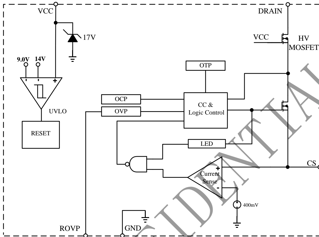
Figure 3. BP2832A Internal Block Diagram
