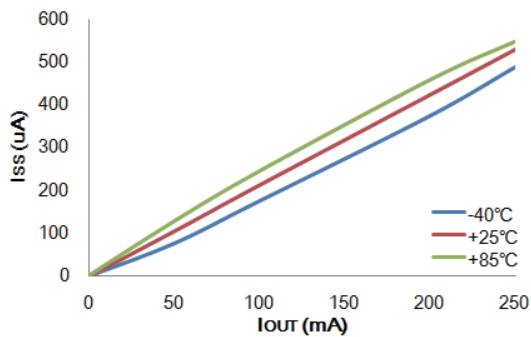
I SS vs I OUT : HT73L27 (V IN =3.7V)
