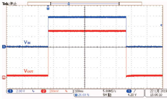
Power On/OFF Response: HT73L09 ( V_{IN}=6.0V , I_{OUT}=0mA , T_{RISE}=T_{FALL}=0.1ms )
