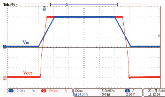
Power On/OFF Response: HT73L30 (V_{IN}=6.0V, I_{OUT}=0mA, T_{RISE}=T_{FALL}=100ms)
