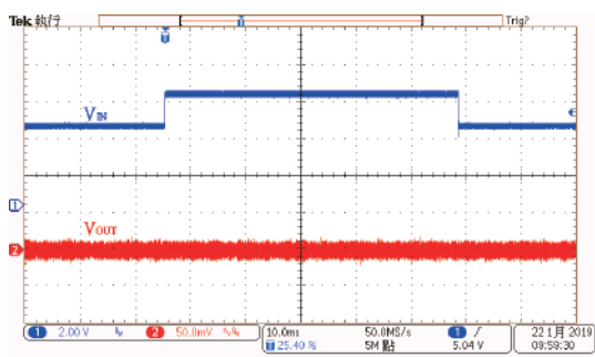
Line Transient Response: HT73L33 ( V_{IN}=4.3V to 6.0V , I_{OUT}=10mA )
