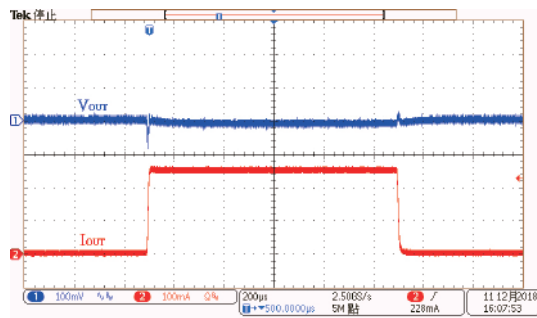
Load Transient Response: HT73L25 ( V_{IN}=3.5V , I_{OUT}=1mA to 250mA )
