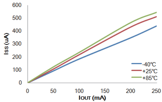
I SS vs I OUT : HT73L25 (V IN =3.5V)
