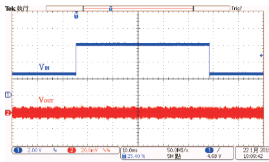
Line Transient Response: HT73L15 ( V_{IN}=2.5V to 6.0V , I_{OUT}=10mA )
