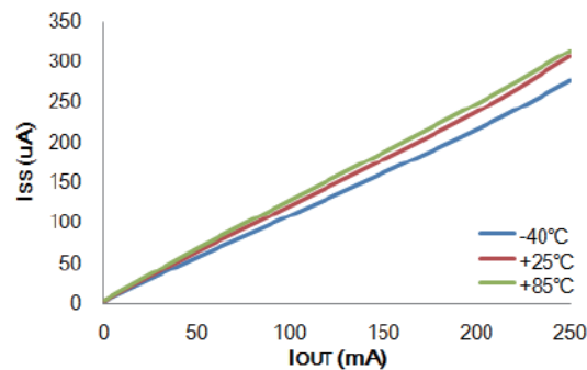
I SS vs I OUT : HT73L30 (V IN =4.0V)
