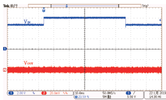
Line Transient Response: HT73L36 ( V_{IN}=4.6 to 6.0V , I_{OUT}=10mA )
