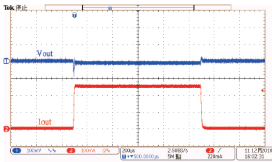
Load Transient Response: HT73L12 ( V_{IN}=2.3V , I_{OUT}=1mA to 250mA )
