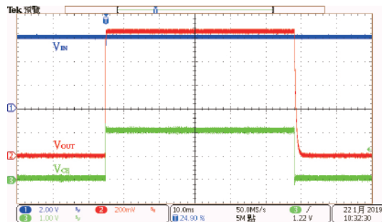
ON/OFF Response: HT73L10 (V_{IN}=6.0V, I_{OUT}=0mA, V_{CE}=0V \text{ to } 2V)
