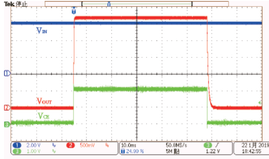
ON/OFF Response: HT73L27 (V_{IN}=6.0V, I_{OUT}=0mA, V_{CE}=0V \text{ to } 2V)
