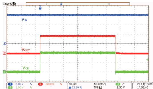
ON/OFF Response: HT73L09 (V_{IN}=6.0V, I_{OUT}=0mA, V_{CE}=0V \text{ to } 2V)
