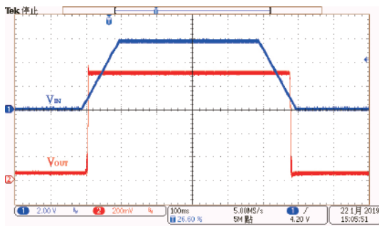
Power On/OFF Response: HT73L09 ( V_{IN}=6.0V , I_{OUT}=0mA , T_{RISE}=T_{FALL}=100ms )
