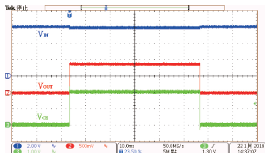
ON/OFF Response: HT73L09 (V_{IN}=6.0V, I_{OUT}=200mA, V_{CE}=0V \text{ to } 2V)
