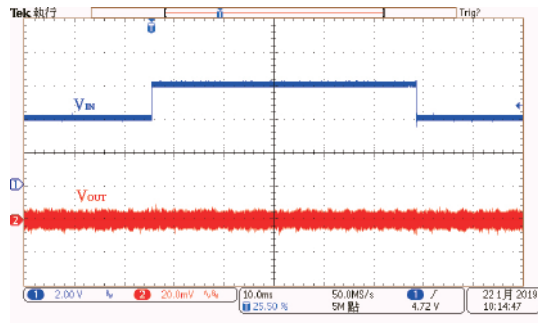
Line Transient Response: HT73L30 ( V_{IN}=3.5V to 6.0V , I_{OUT}=10mA )
