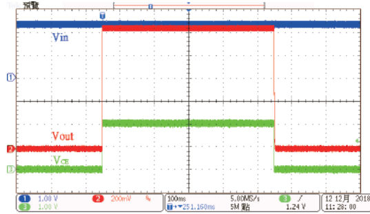
ON/OFF Response: HT73L10 (V_{IN}=2.3V, I_{OUT}=0mA, V_{CE}=0V \text{ to } 2V)
