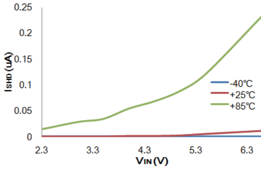
I SHD vs V IN : HT73L12 (I OUT =0mA)
