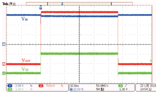
ON/OFF Response: HT73L27 (V_{IN}=6.0V, I_{OUT}=200mA, V_{CE}=0V \text{ to } 2V)
