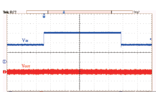
Line Transient Response: HT73L25 ( V_{IN}=3.5V to 6.0V , I_{OUT}=10mA )
