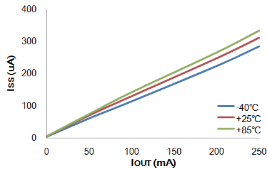
I SS vs I OUT : HT73L36 (V IN =4.6V)
