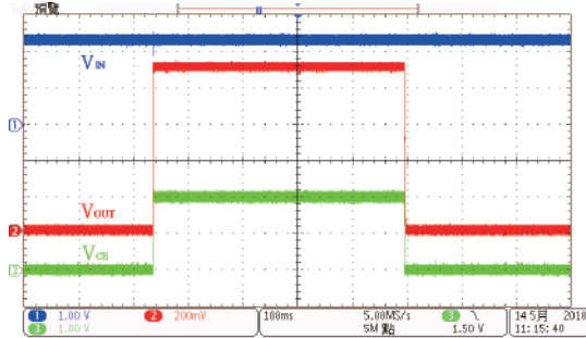
ON/OFF Response: HT73L09 (V_{IN}=2.3V, I_{OUT}=0mA, V_{CE}=0V \text{ to } 2V)
