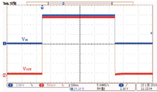
Power On/OFF Response: HT73L30 (V_{IN}=6.0V, I_{OUT}=0mA, T_{RISE}=T_{FALL}=0.1ms)
