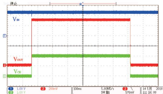
ON/OFF Response: HT73L09 (V_{IN}=2.3V, I_{OUT}=200mA, V_{CE}=0V \text{ to } 2V)
