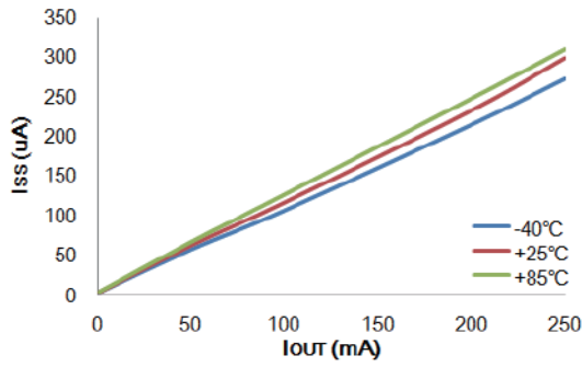
I SS vs I OUT : HT73L12 (V IN =2.3V)
