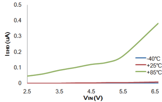
I SHD vs V IN : HT73L15 (I OUT =0mA)
