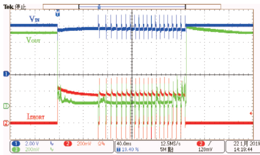
Short Protection: HT73L09 ( V_{IN}=6.0V , V_{OUT} Short)
