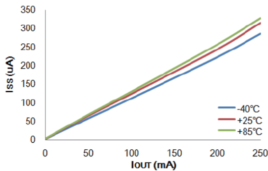
I SS vs I OUT : HT73L33 (V IN =4.3V)
