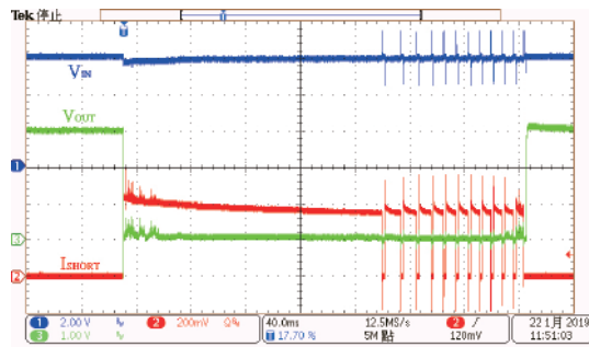
Short protection: HT73L30 ( V_{IN}=6.0V , V_{OUT} short)
