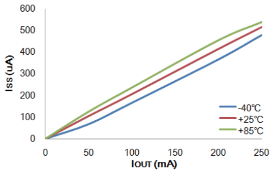
I SS vs I OUT : HT73L18 (V IN =2.8V)
