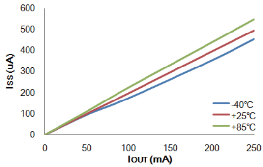
I SS vs I OUT : HT73L15 (V IN =2.5V)
