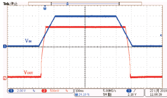
Power On/OFF Response: HT73L25 ( V_{IN}=6.0V , I_{OUT}=0mA , T_{RISE}=T_{FALL}=100ms )
