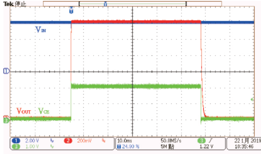
ON/OFF Response: HT73L12 (V_{IN}=6.0V, I_{OUT}=0mA, V_{CE}=0V \text{ to } 2V)
