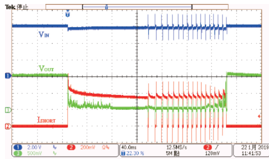
Short Protection: HT73L10 ( V_{IN}=6.0V , V_{OUT} Short)
