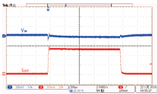
Load Transient Response: HT73L33 ( V_{IN}=6.0V , I_{OUT}=1mA to 250mA)
