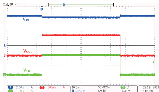
ON/OFF Response: HT73L10 (V_{IN}=6.0V, I_{OUT}=200mA, V_{CE}=0V \text{ to } 2V)
