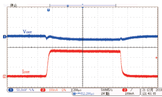
Load Transient Response: HT73L36 ( V_{IN}=6.0V , I_{OUT}=1mA to 250mA)
