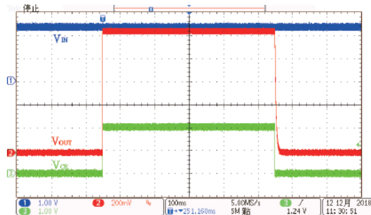
ON/OFF Response: HT73L10 (V_{IN}=2.3V, I_{OUT}=200mA, V_{CE}=0V \text{ to } 2V)
