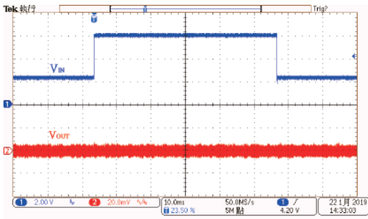
Line Transient Response: HT73L09 ( V_{IN}=2.3V to 6.0V, I_{OUT}=10mA )
