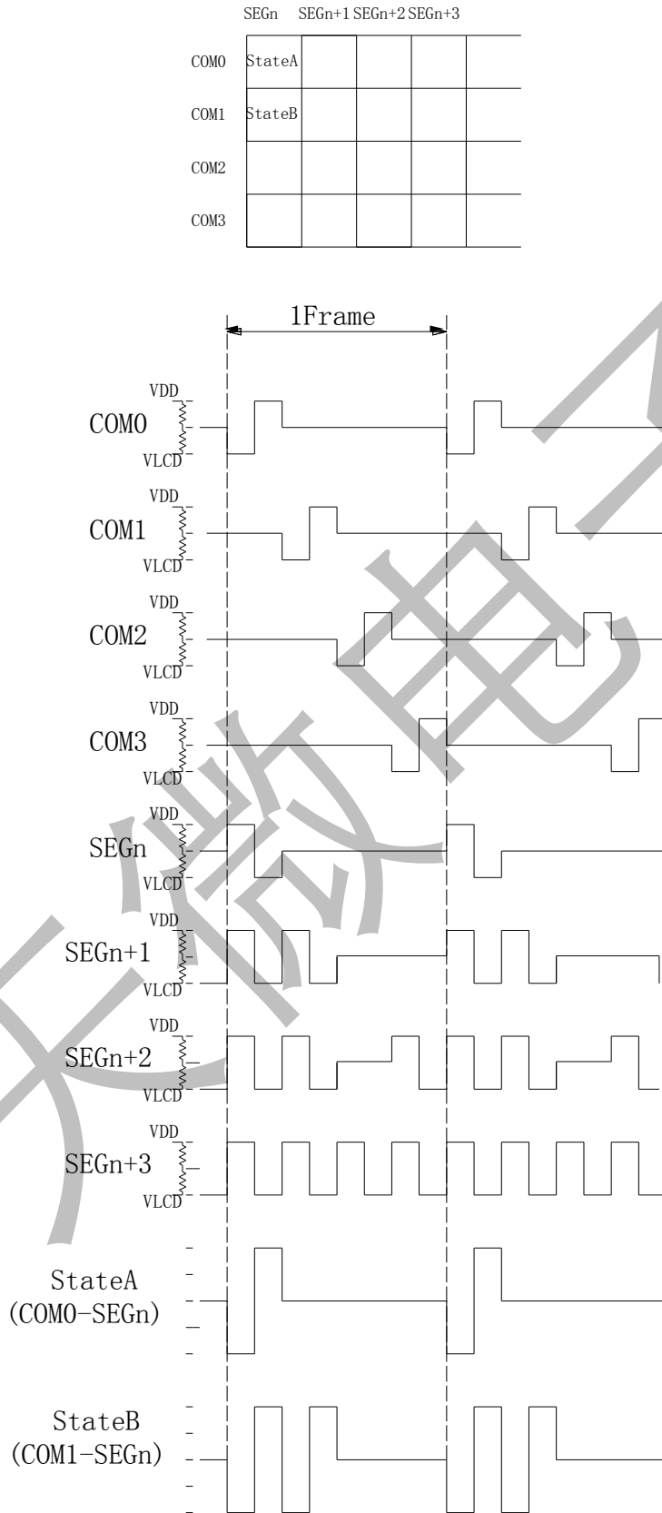
(3) 1/2Bias, Line翻转的液晶驱波形
