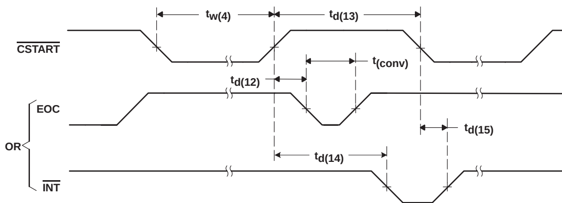
Figure 4. Critical Timing for Extended Sampling ( \overline{\text{CSTART}} Trigger)
