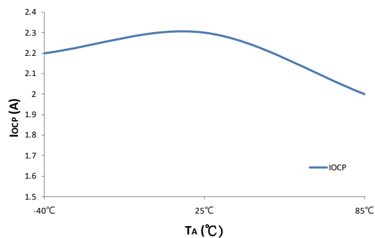
I_{OCP} vs. Temperature
