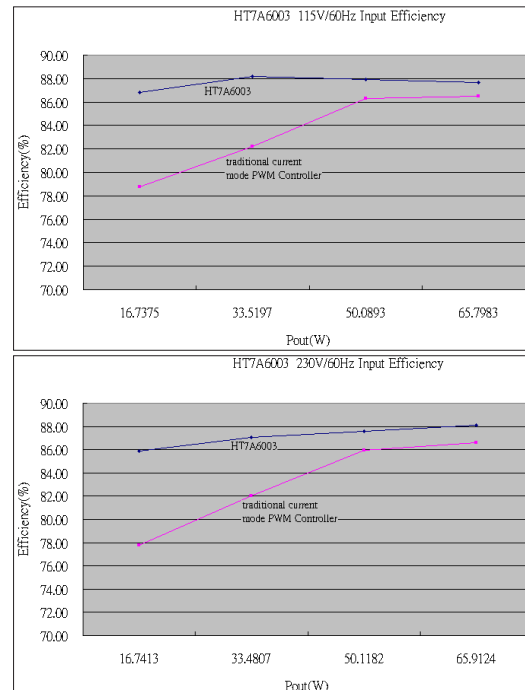
Figure 8. Efficiency Comparison between HT7A6003 & Traditional Current Mode PWM Controller (Measured at HT7A3942 Demo Board)
