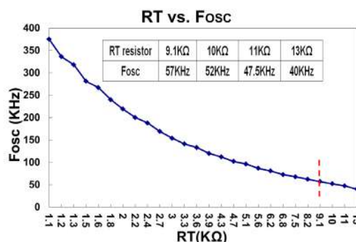
Figure 14. RT Resistor value vs Operating Frequency
