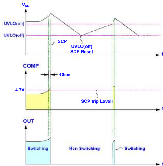
Figure 12. SCP Function Behavior
