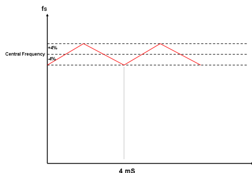
Figure 13. Frequency Jitter Function Spreads Energy Over a Period to Accomplish EMI Restraining
