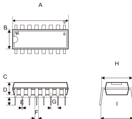
Fig2. 1/2 Lead Packages
