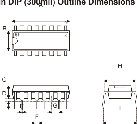
Fig1. Full Lead Packages
