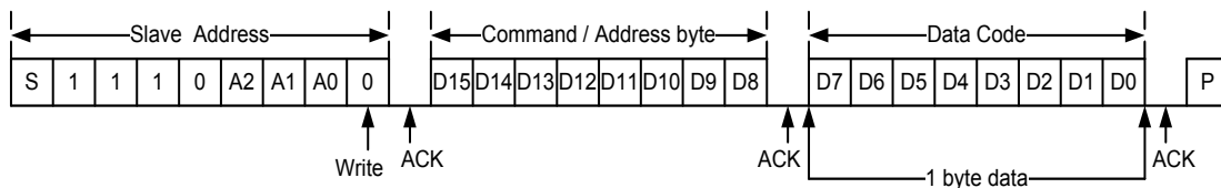
Command and Single Data Byte Received
