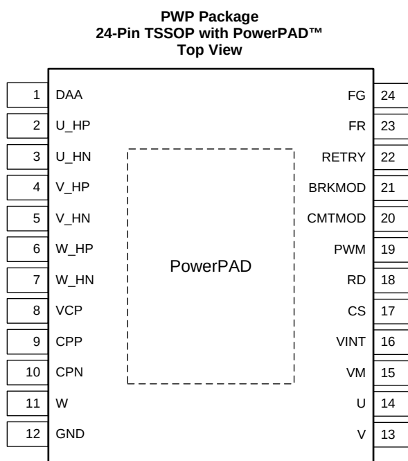
Pin Functions
