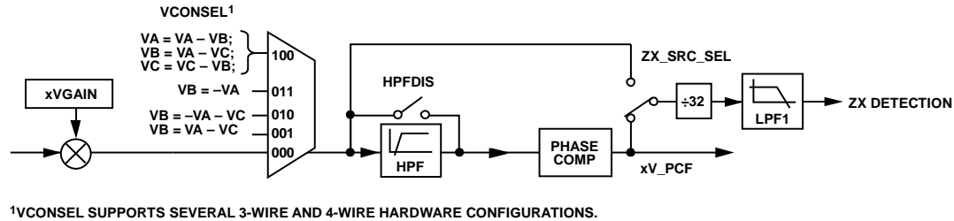
Figure 67. Voltage Channel Signal Chain Preceding Zero-Crossing Detection
