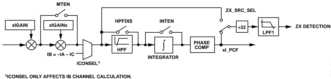
Figure 68. Current Channel Signal Chain Preceding Zero-Crossing Detection
