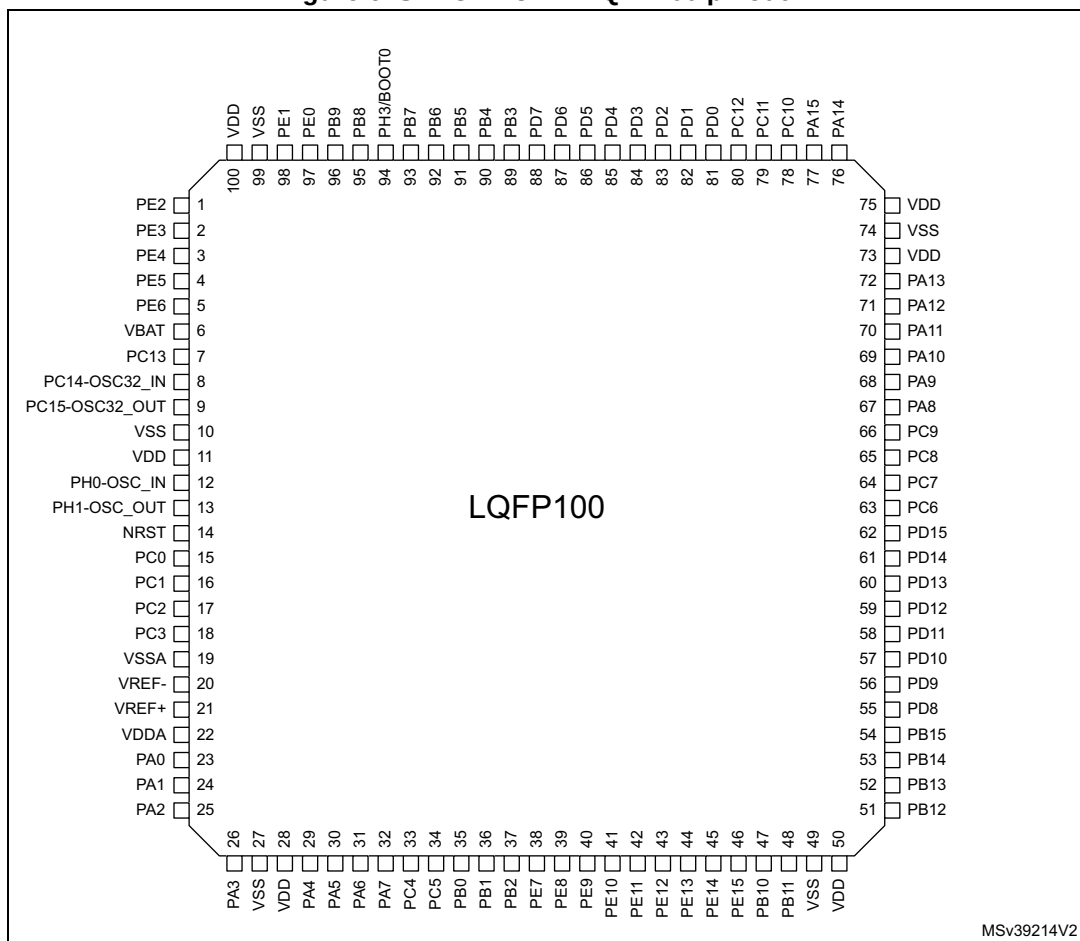
Figure 6. STM32L431Vx LQFP100 pinout (1)
