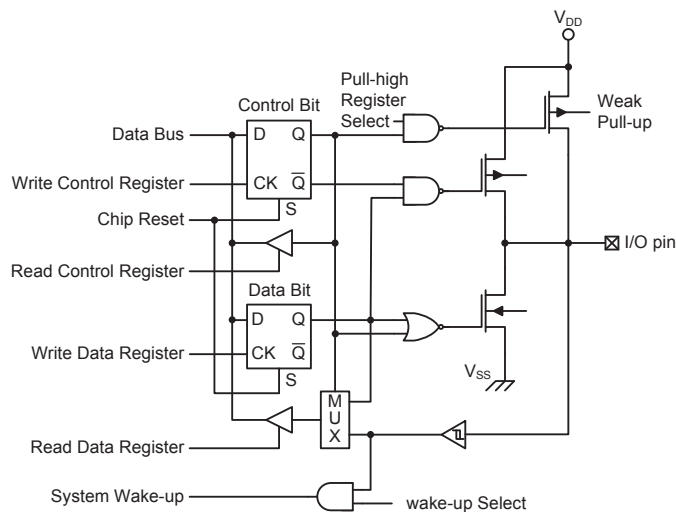
Logic Function Input/Output Structure – PA Port
