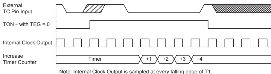
Pulse Width Capture Mode Timing Chart (TEG=0)
