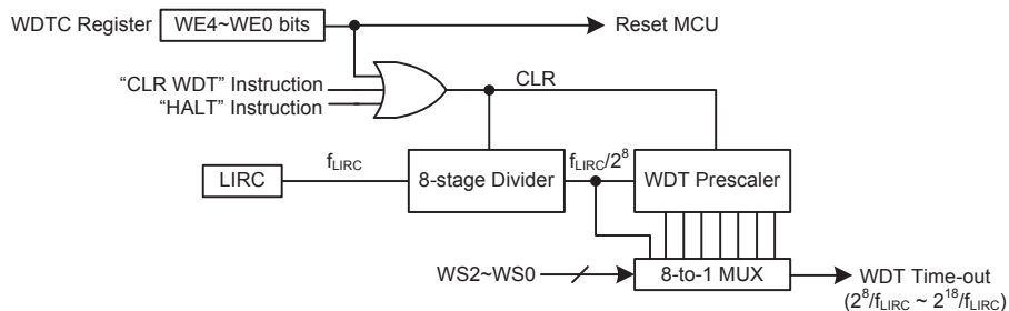
Watchdog Timer
