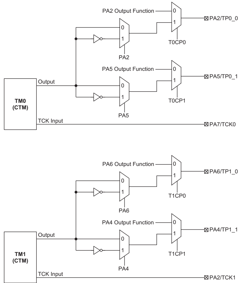
HT66F005/HT66F006 TM Function Pin Control Block Diagram
