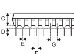
Fig2. 1/2 Lead Packages
