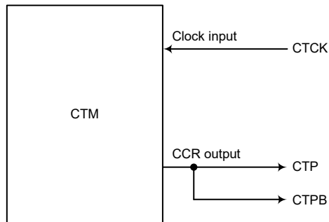
CTM Function Pin Block Diagram
