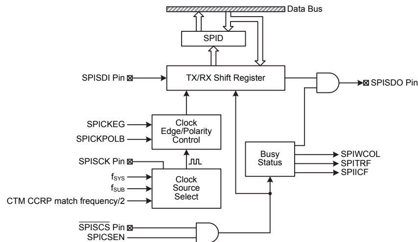
SPI Block Diagram
