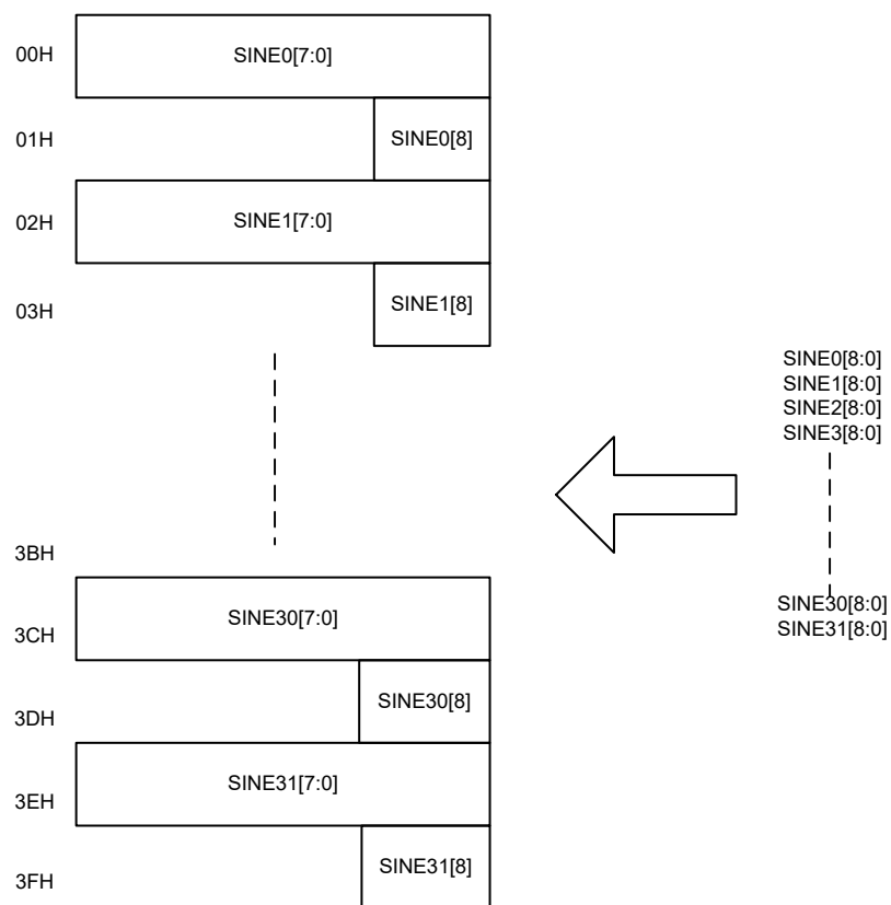
Data memory (Sector 3)
