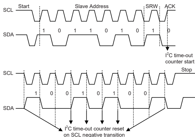
I²C Time-out
