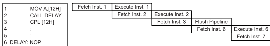
Instruction Fetching
