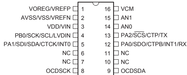
BH66V5232-10 16 NSOP-A
