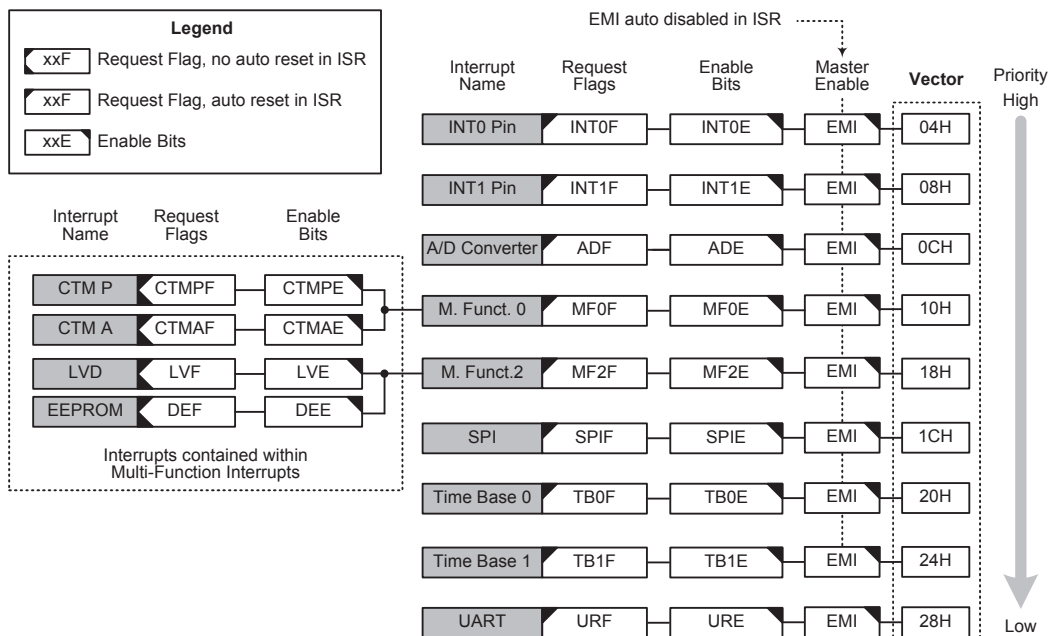
Interrupt Structure – BH66F2652/BH66F2652-2
