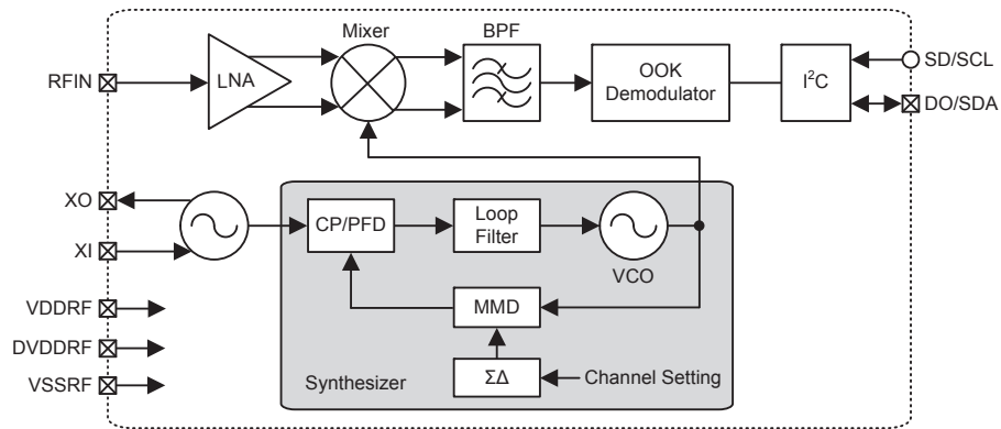
RF Receiver Block Diagram
