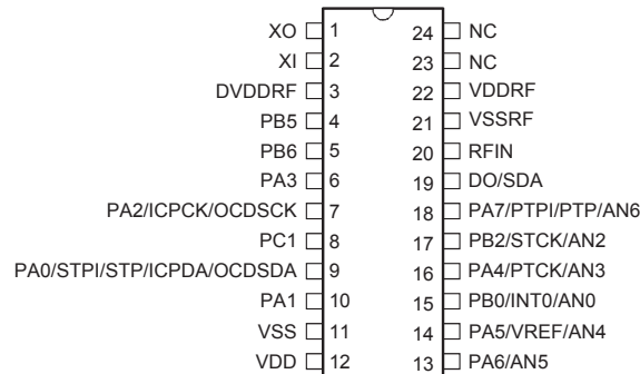
BC66F2342/BC66V2342 24 SSOP-EP-A
